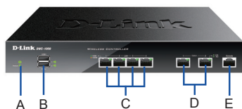
Figura 1. Panel frontal del DWC-1000
