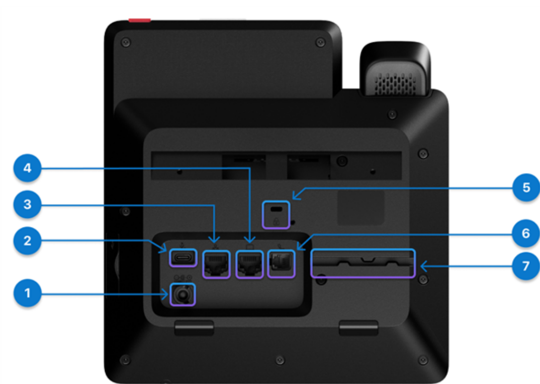
Figure 5. Cisco Desk Phone 9851 back view
