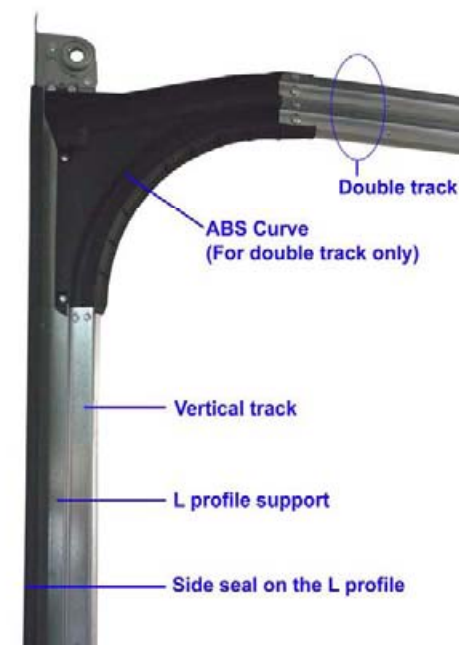
For L Profile with ABS Curve
