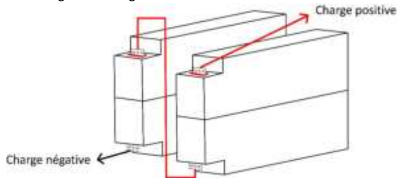
Figure 4.1: Two GC3 Batteries Connected in Series to create a 24V 270Ah Battery Bank
