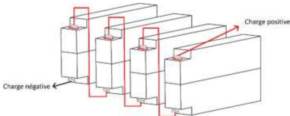
Figure 4.2: Four GC3 Batteries Connected in Series to create a 48V 270Ah Battery Bank
