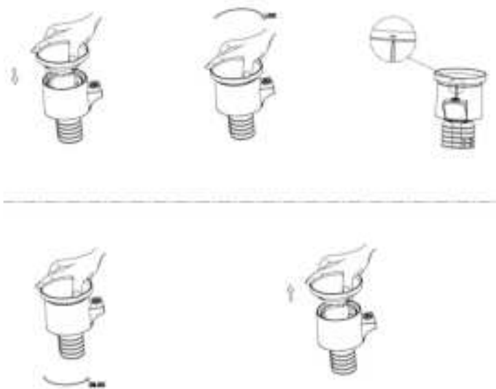
Figure 11 Rain gauge installation and maintenance
