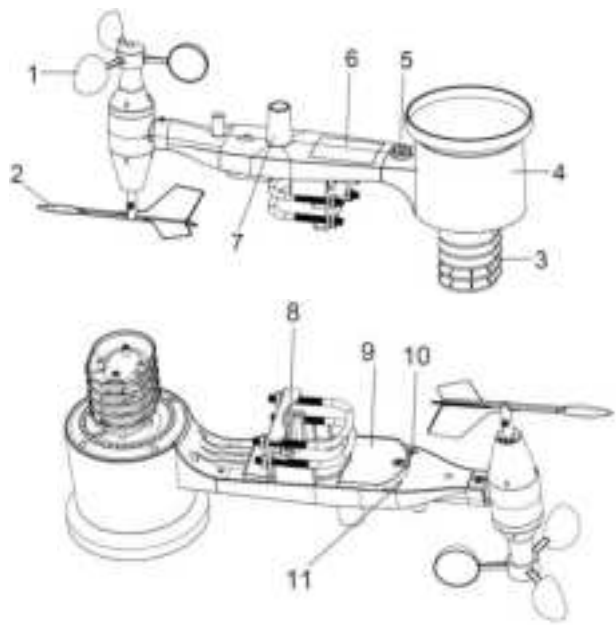
Figure 3 Sensor assembly components
