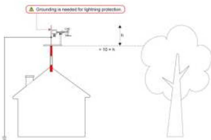
Figure 9 Grounding protection
