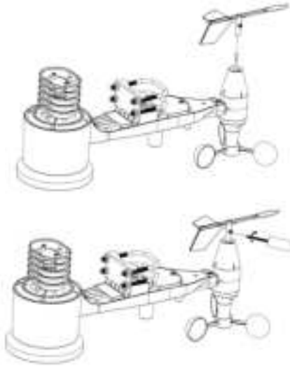
Figure 6 Wind vane installation diagram
