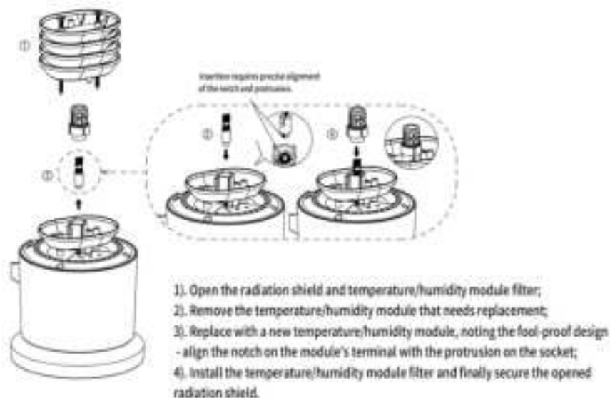
Figure 12 Temperature and humidity module installation
