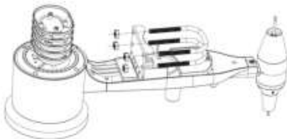
Figure 4 U-Bolt installation
