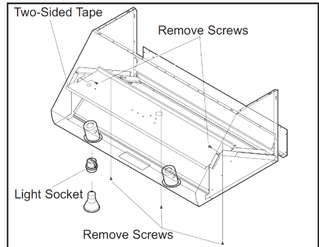
Figure 3-10 (cutaway view).
