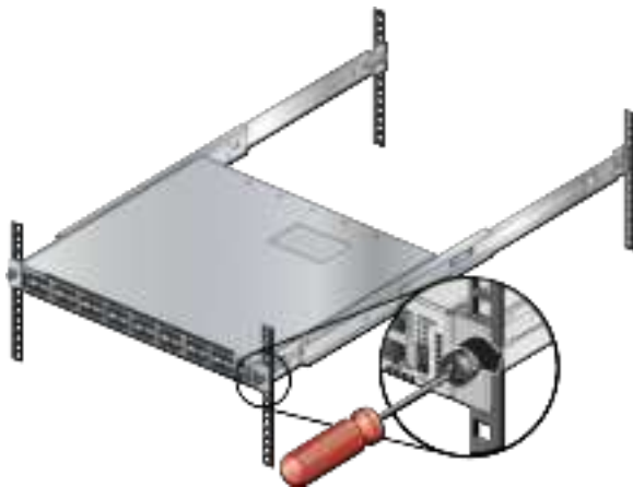
Figure 3-13: Attaching the Switch to the Rack Posts
