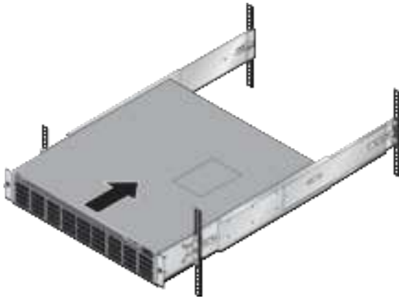
Figure 3-18: Inserting the Switch onto the Rails
