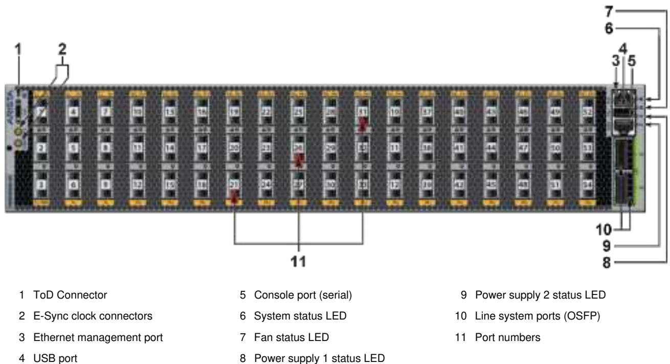
Figure C-1: DCS-7280DR3A-54, DCS-7280DR3AK-54, and DCS-7280DR3AM-54
