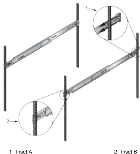
Figure 3-11: Attaching the Rails
