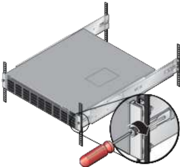
Figure 3-19: Attaching the Switch to the Rack Posts
