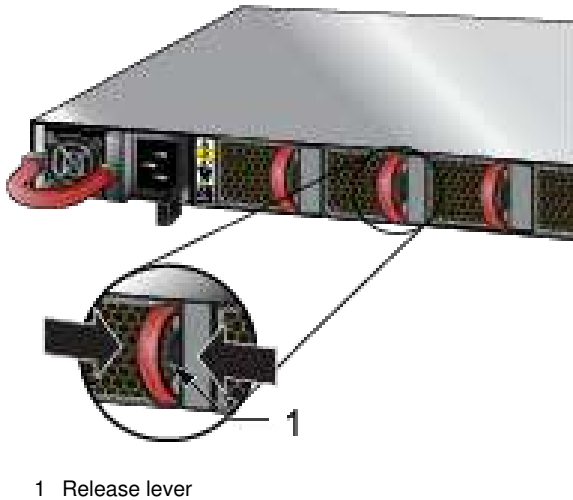
Figure E-2: Removing Fan Module
