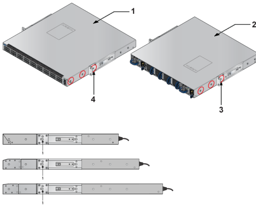
Figure 3-1: Bracket Mount Examples for Two-Post Rack Mount
