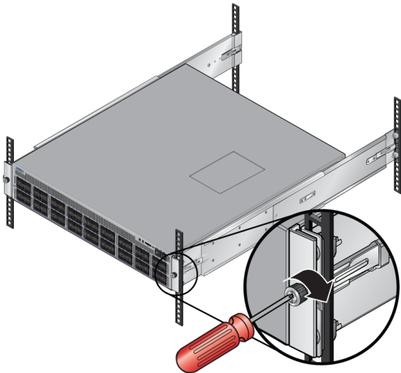
Figure 3-19: Attaching the Switch to the Rack Posts
