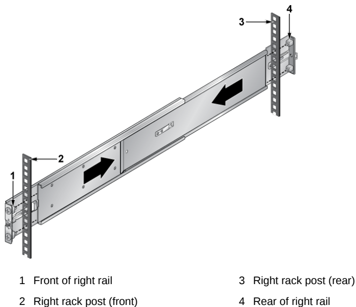
Figure 3-17: Attaching the Rails
