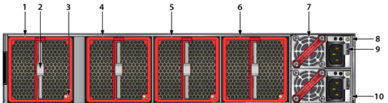
Figure D-4: Rear Panel with Separation Between Fans 1 and 2 (no ground)
