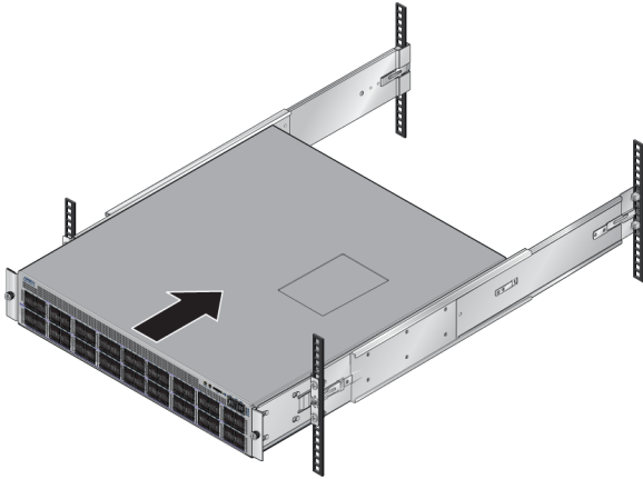
Figure 3-18: Inserting the Switch onto the Rails
