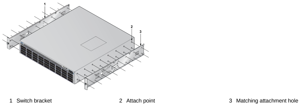
Figure 3-15: Front Bracket Alignment
