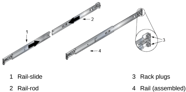
Figure 3-10: Assembling the Rails
