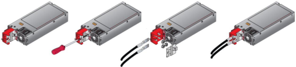
Figure 4-7: DC PSU Connection Example
