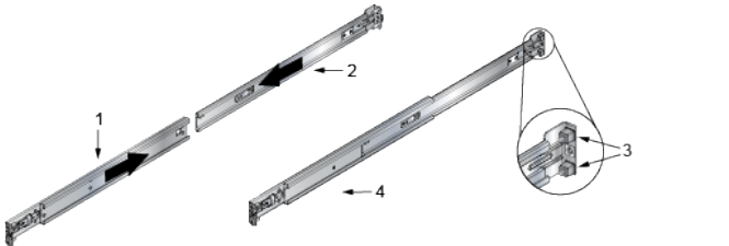
1 Rail-slide 2 Rail-rod 3 Rack plugs (detail) 4 Rail (assembled)
