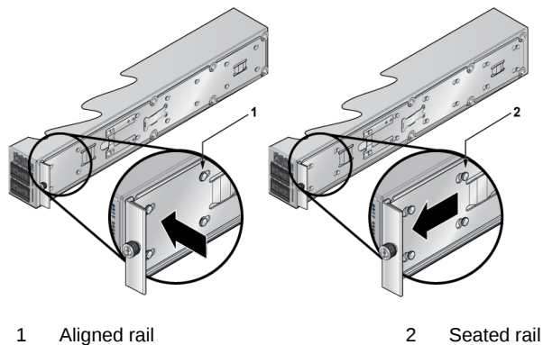
Figure 3-16: Attaching the Mounting Brackets to the Switch Chassis
