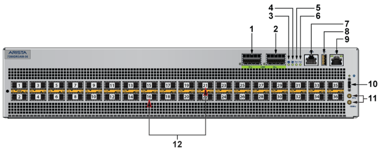
Figure C-2: DCS-7280DR3A-36, DCS-7280DR3AK-36, and DCS-7280DR3AM-36
