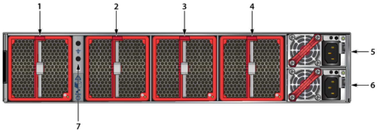
Figure D-3: Rear Panel with Ground Attach Point (2RU)
