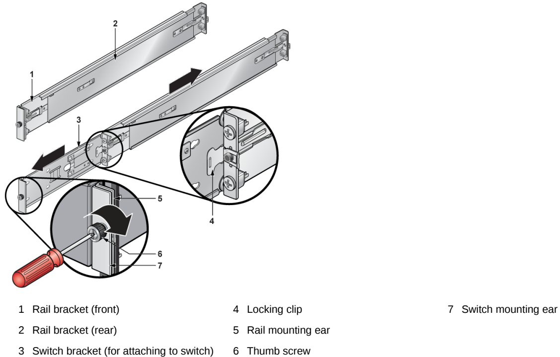
Figure 3-14: Accessory Kit Components
