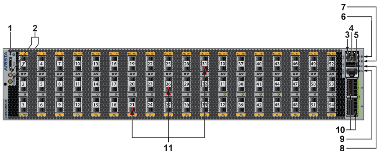
Figure C-1: DCS-7280DR3A-54, DCS-7280DR3AK-54, and DCS-7280DR3AM-54
