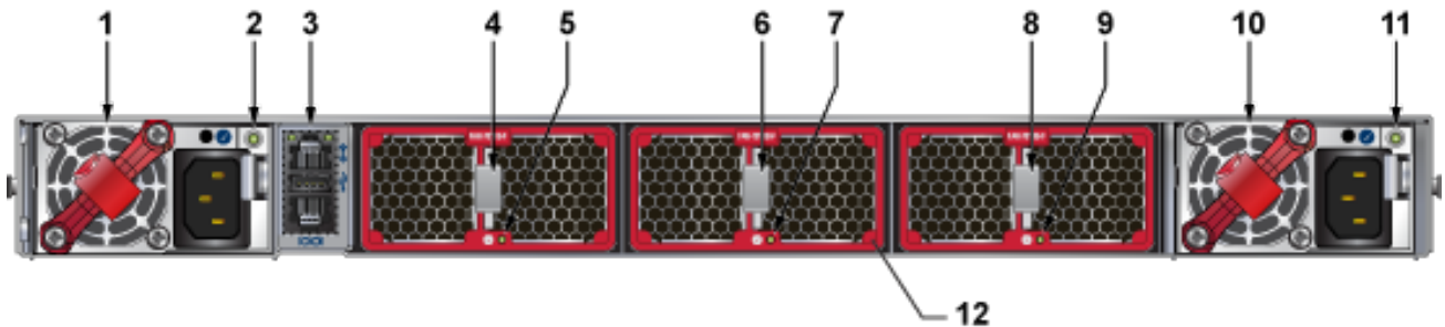
Figure D-2: Rear Panel with Three Fan Modules (1RU)
