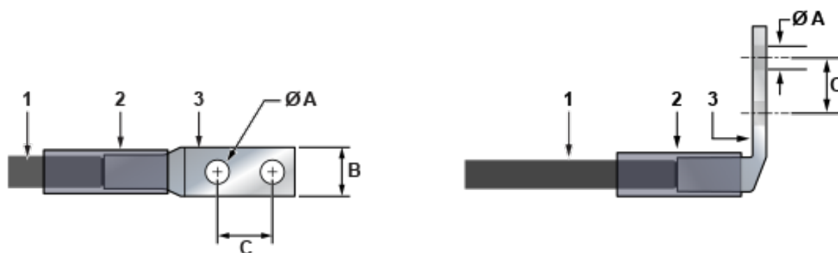
Figure 4-6: Lug Preparation
