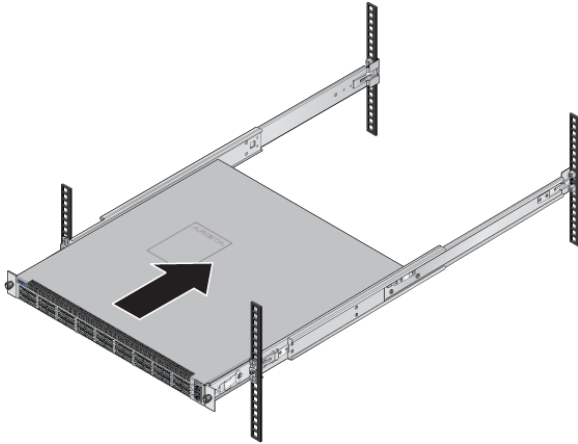
Figure 3-12: Inserting the Switch onto the Rails
