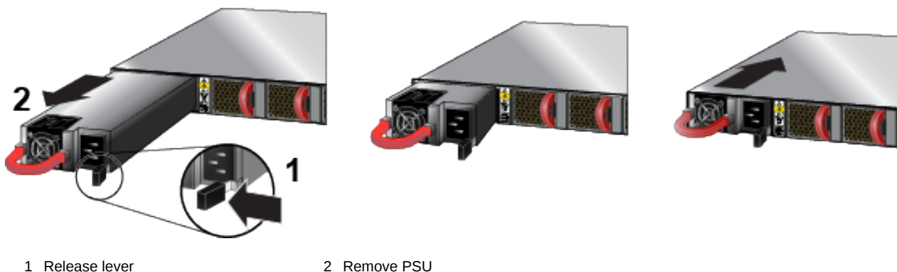
Figure E-1: Removing and Installing Power Supply
