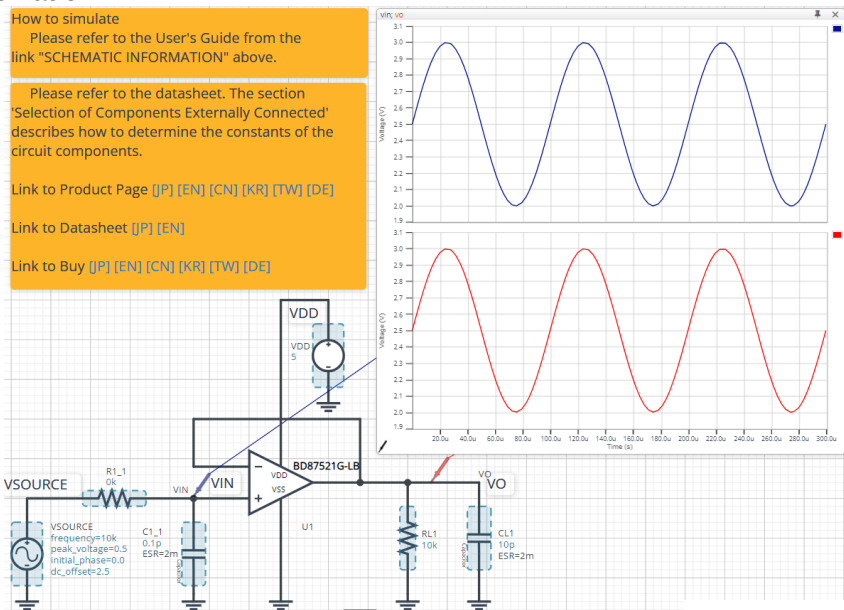
Figure 1. Simulation Schematic
