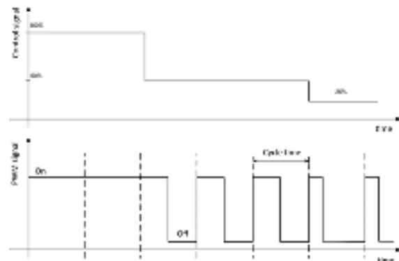
Fig. 04-3 Control signal and corresponding PWM signal
