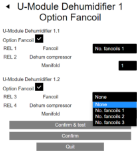
Fig. 07-24 Webpage: U-Module for dehumidifier and switched Fan Coils
