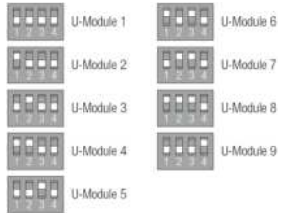
Fig. 07-3 DIP switches on U-Module
