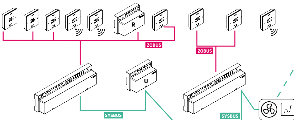
Fig. 05-1 Zone Bus (ZOBUS) and System Bus (SYSBUS)
