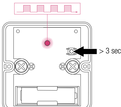
Fig. 07-5 Pairing outdoor sensor
