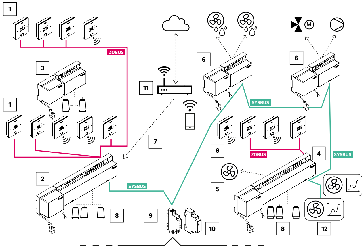
Fig. 03-2 System overview NEA SMART 2.0 24 V
