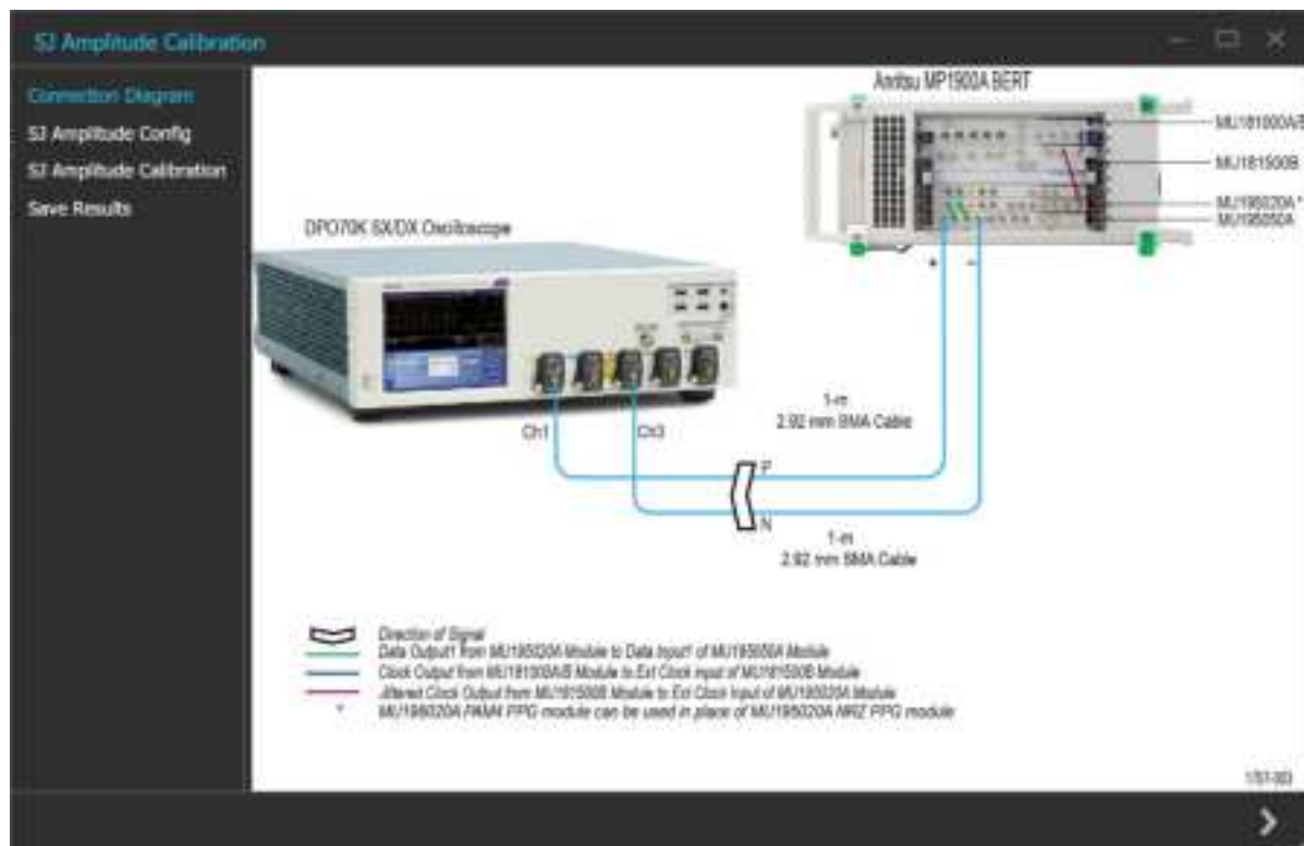
Figure 10: SJ Amplitude Calibration - Connection diagram
