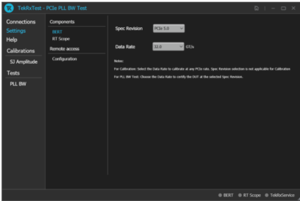
Figure 6: Settings panel
