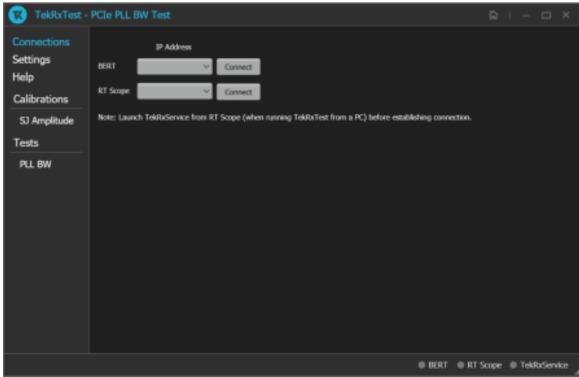
Figure 5: Connections panel
