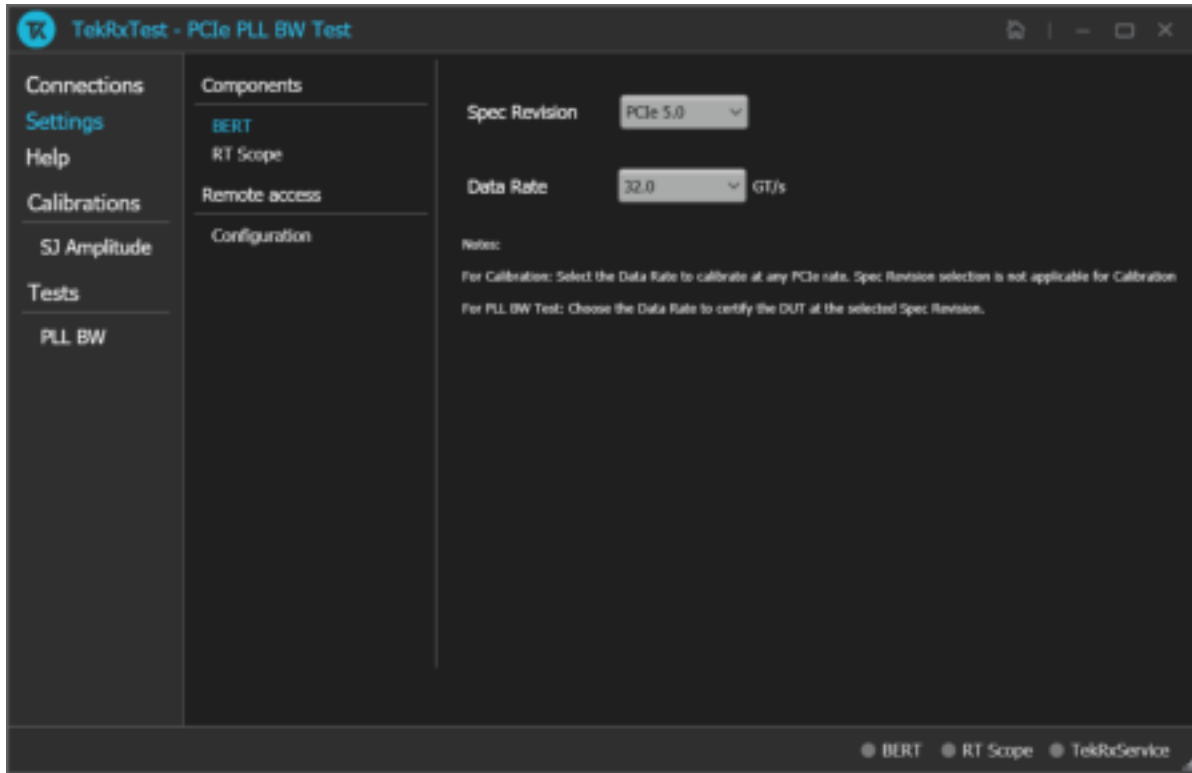
Figure 7: Components: BERT
