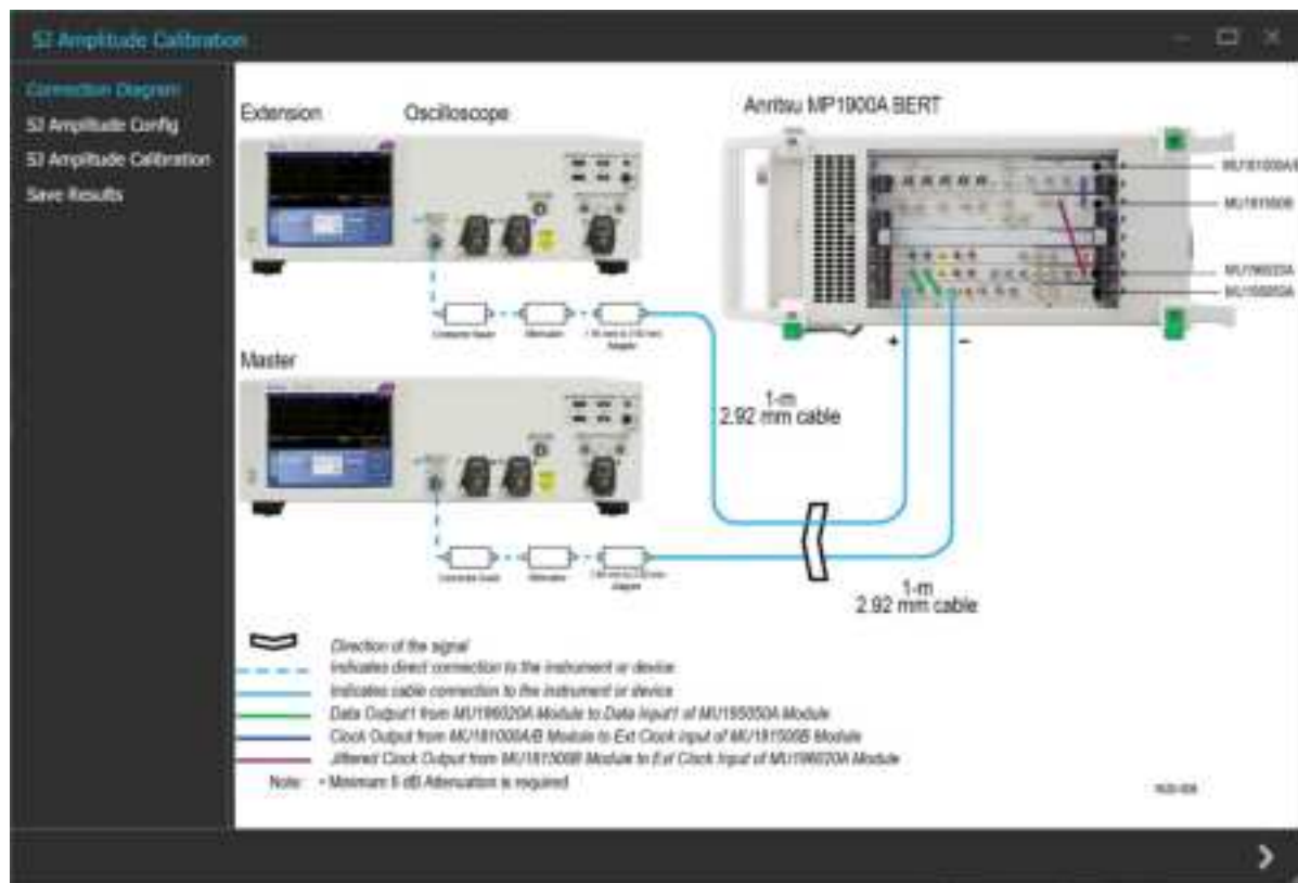
Figure 11: SJ Amplitude Calibration for 200 GS/s - Connection Diagram
