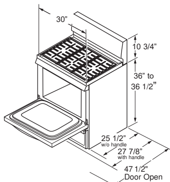
REAR CONTROL
