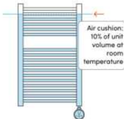
Figure 6 | Air cushion requirement (image for illustrative purposes only)
