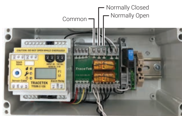
Figure 5. Alarm Relay Connections
