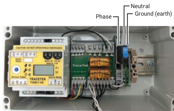
Figure 3. Power connections
