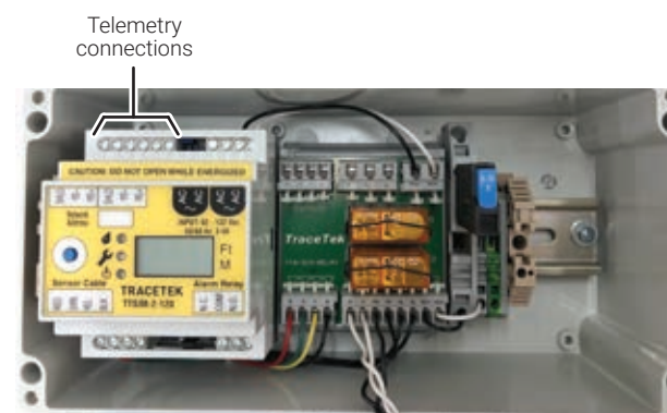
Figure 6. Telemetry Connections
