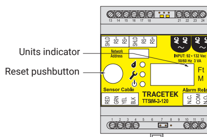
Figure 11. RESET pushbutton and units indicator locations
