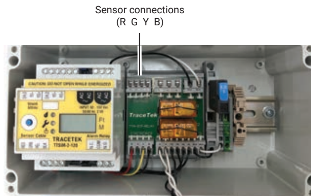
Figure 4. Sensor Connections
