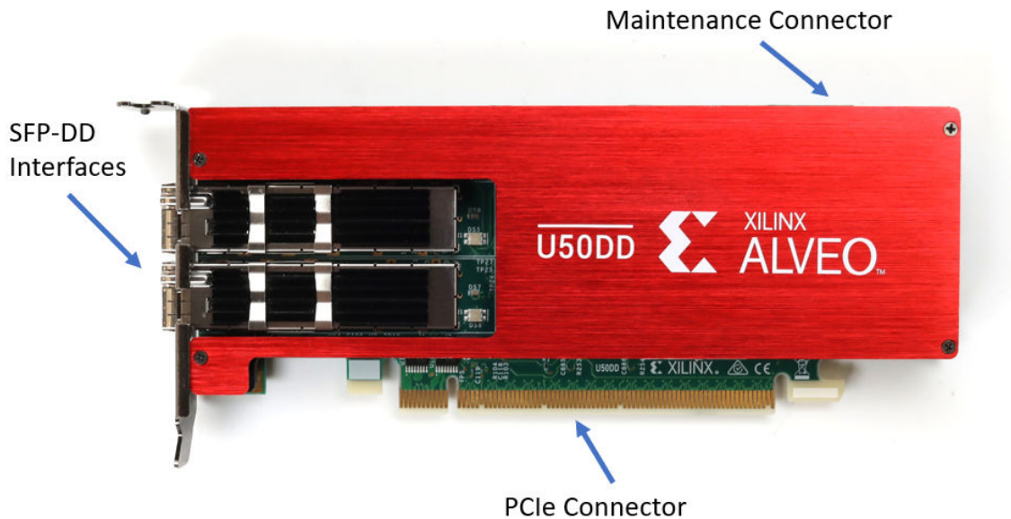
Figure 2: Alveo U50DD ES Card with Half-Height Bracket
