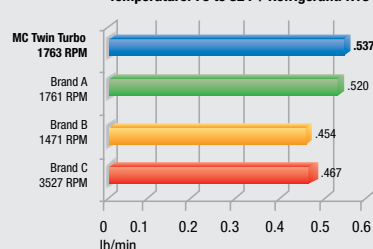
Vapor Recovery (Out) lb/min • Temperature: 79 to 82°F / Refrigerant: R134a
