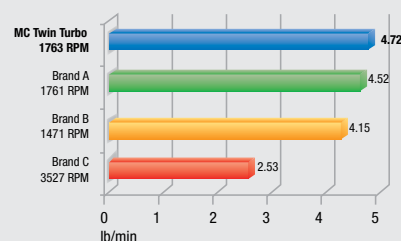
Vapor Recovery (Out) lb/min • Temperature: 79 to 82°F / Refrigerant: R134a
