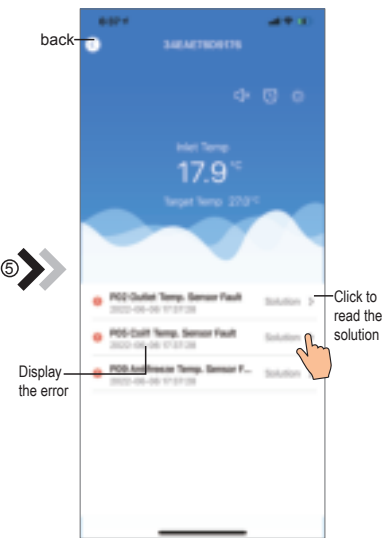
Fig.43 Troubleshooting interface
