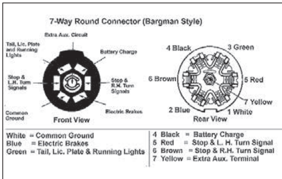
Figure 9-12: Seven-Pin towing connector
