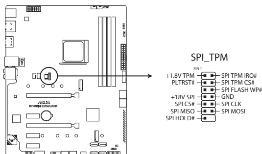
TUF GAMING X570-PLUS/BR SPI_TPM connector
