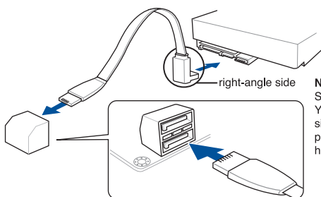
TUF GAMING X570-PLUS/BR SATA 6 Gb/s connectors
