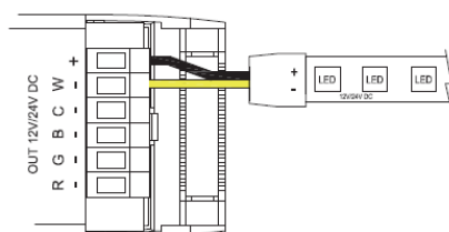
Output wiring of dual color LED strip
