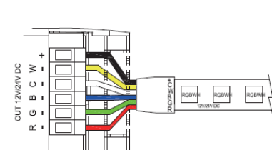
Output wiring of RGB+CW+WW LED strip
