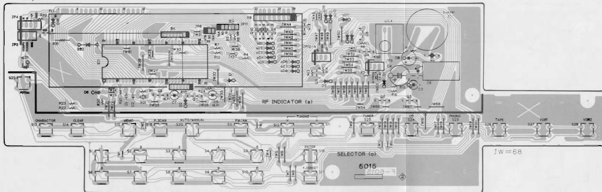
5-5. F-6015 Display and Operation Switch Board
