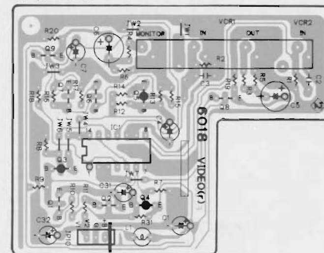
5-8. F-6018 Video In/Out Terminal Board
