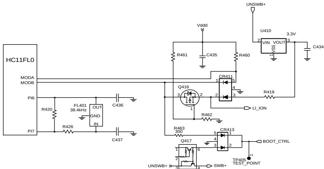
Figure 4-3: RTC Circuit
