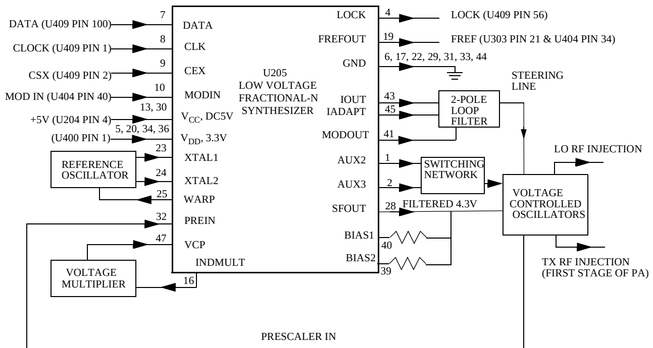
Figure 6-4: Lowband Synthesizer Block Diagram
