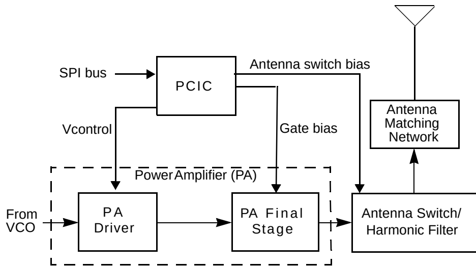
Figure 6-1: Lowband Transmitter Block Diagram
