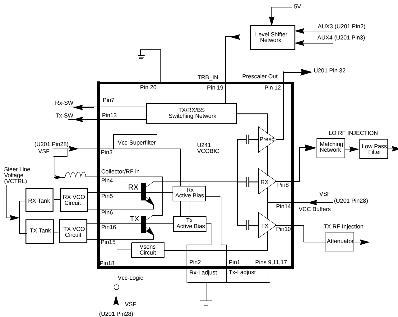
Figure 6-5 VCO Block Diagram
