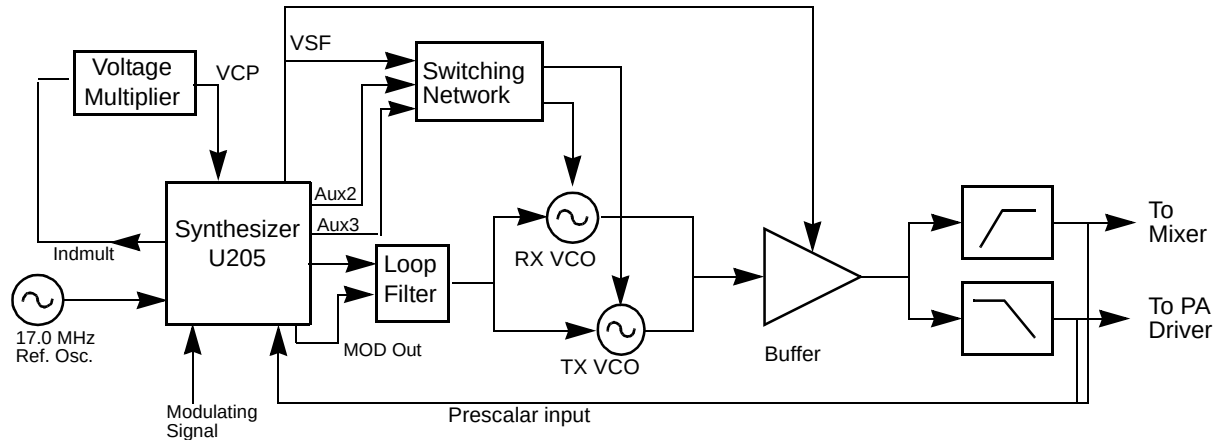
Figure 6-3: Lowband Frequency Generation Unit Block Diagram
