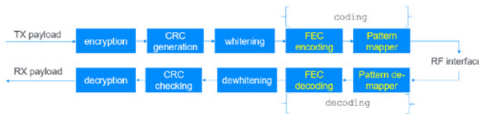
Figure 5 - FEC in Bluetooth 5 bit stream processing
