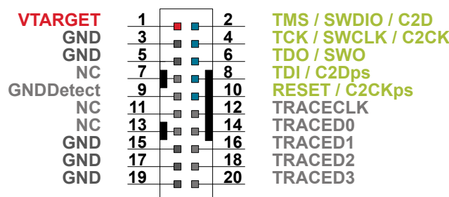
Figure 3.4. Debug Connector
