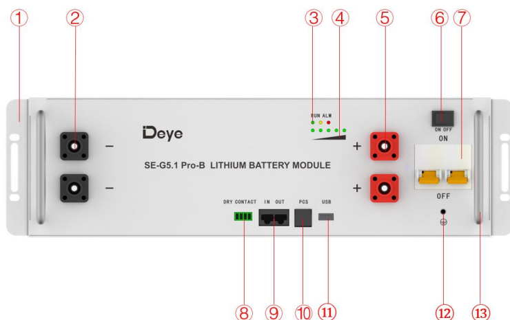
Figure 2-1: Front Panel Function Introduction
