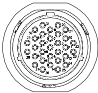
RECEPTACLE CONNECTOR FREE HANGING
