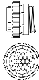
PLUG CONNECTOR
