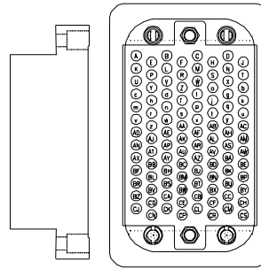
104 PIN RECTANGULAR PLUG CONNECTOR
