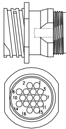
RECEPTACLE CONNECTOR FREE HANGING
