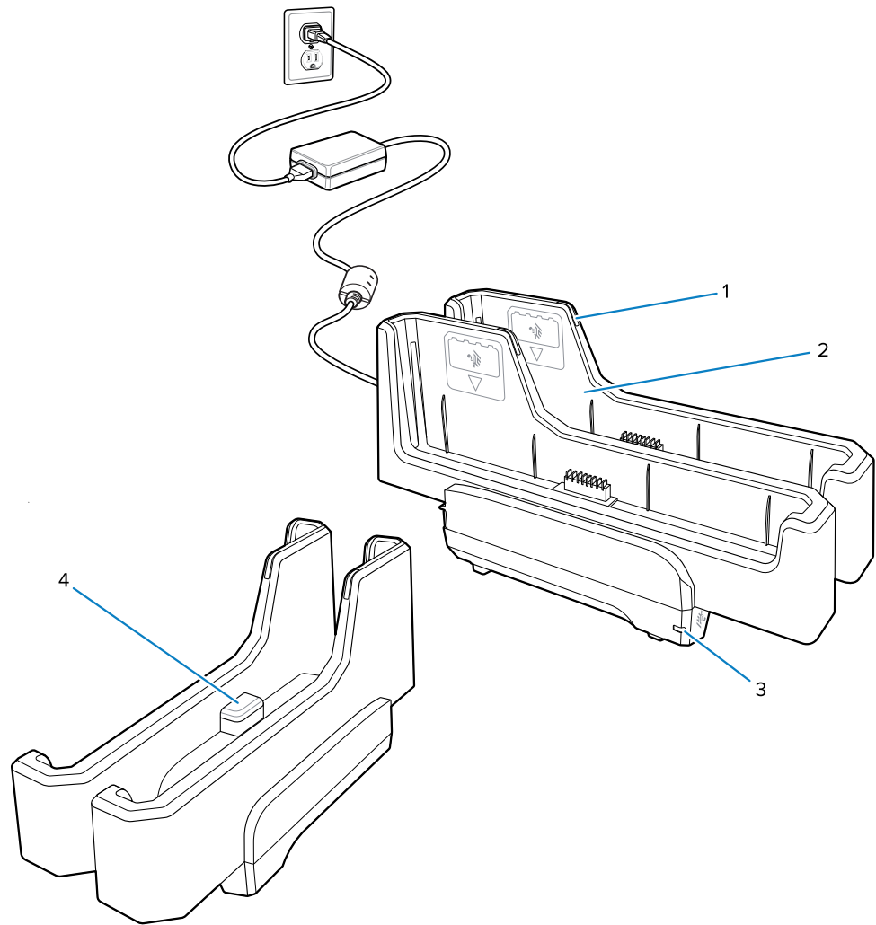
Figure 5 2-Slot Battery Charger
