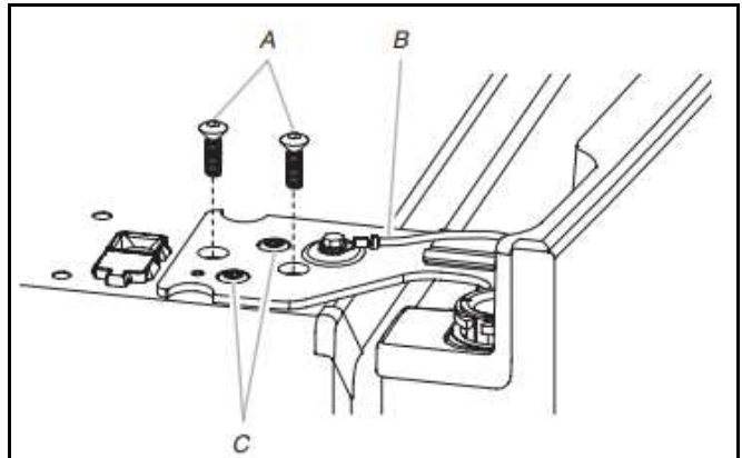
A. 3/4" Internal hex-head or TORX T25 screws
