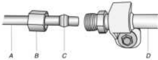
A. Household water line C. Ferrule (purchased) B. Nut (purchased) D. Refrigerator water tubing
