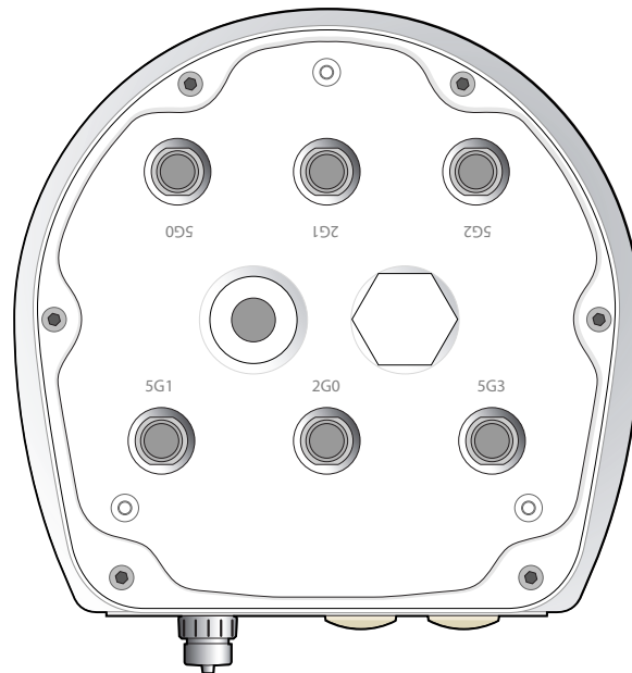
Figure 8 AP-374 Bottom View (without Aesthetic Cover)
