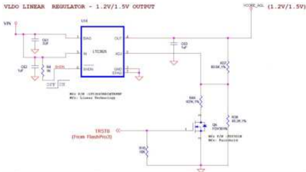
Figure 13-1 • Circuit Diagram
