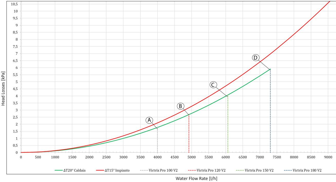
Single boiler plate exchanger kit pressure drop graphVICTRIX PRO V2 100-120-150-180 EU \Delta T20^\circ Primary/ \Delta T15^\circ Secondary
