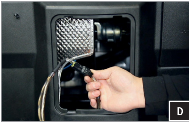
D. From the rear of the center console, route the B-H1150 harness up to each speaker pod and connect.
