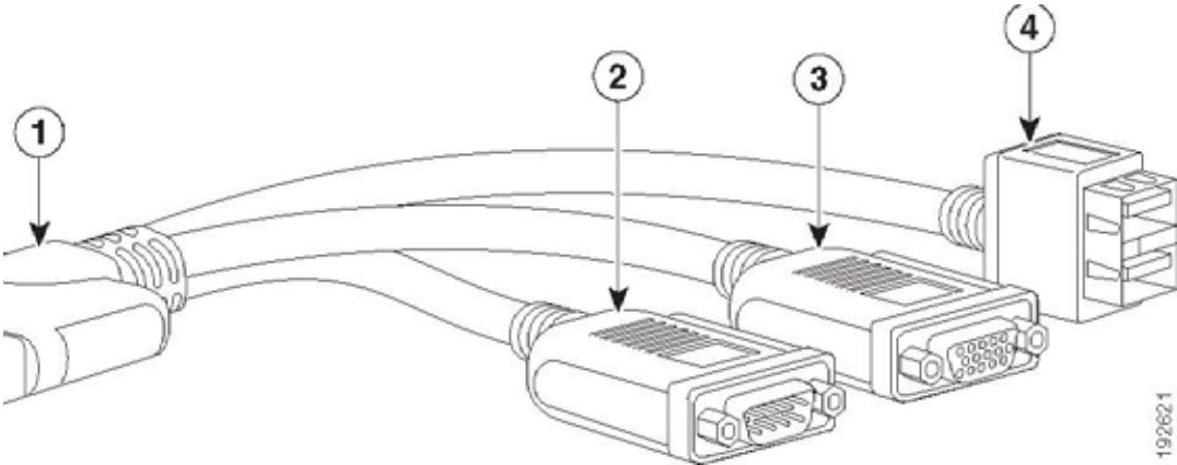
Figure 7 KVM Cabbble
