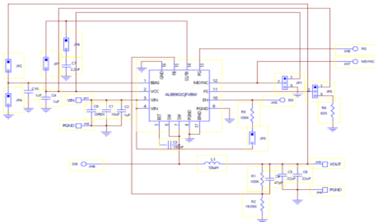
Figure 6: Schematic Circuit
