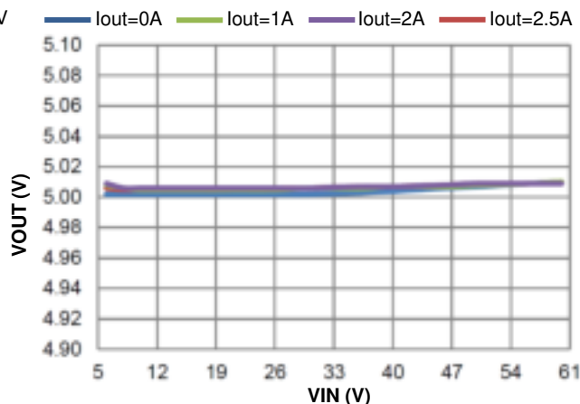
Figure 8. PWM Line Regulation
