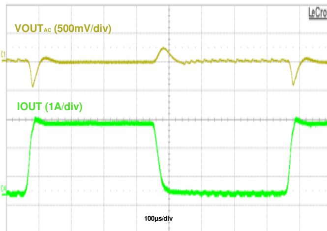
Figure 12. Load Transient, I OUT = 50mA to 2.5A to 50mA, PFM
