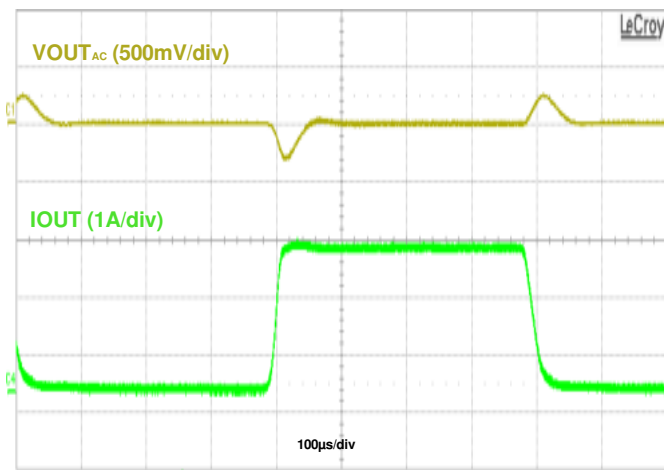
Figure 11. Load Transient, I OUT = 50mA to 2.5A to 50mA, PWM
