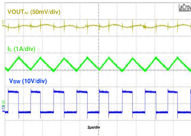
Figure 9. Output Ripple, VIN=12V, V OUT = 5V @2.5A, PWM
