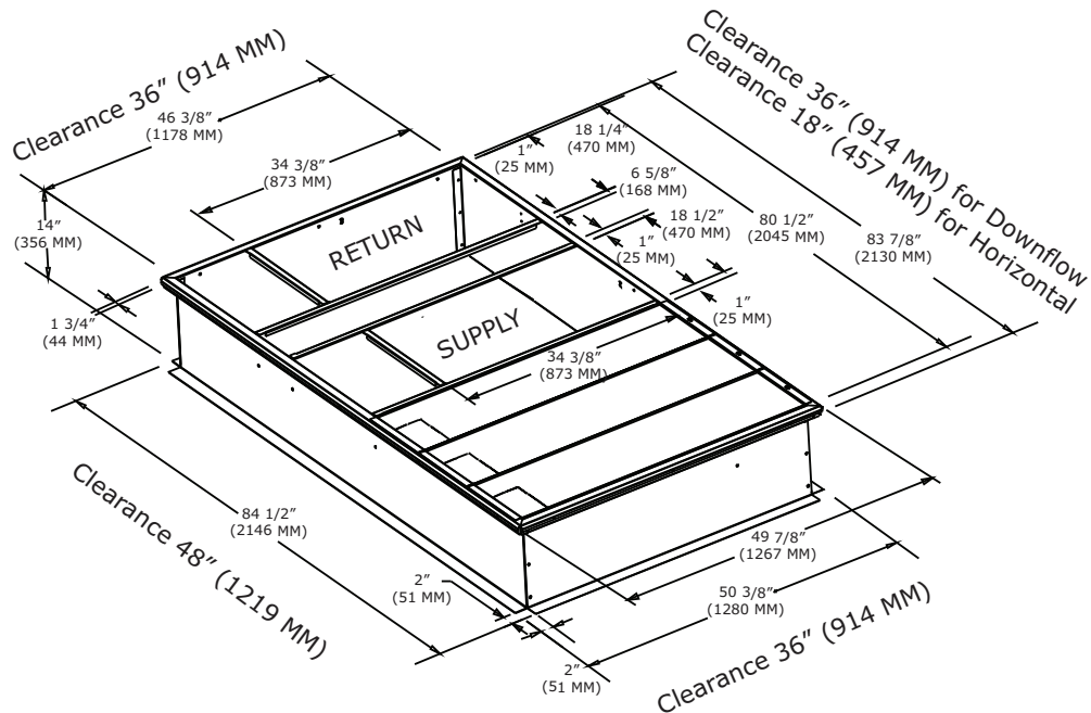
Figure 18. Cooling and gas/electric - 4 to 5 tons ultra high efficiency - roof curb (a)
