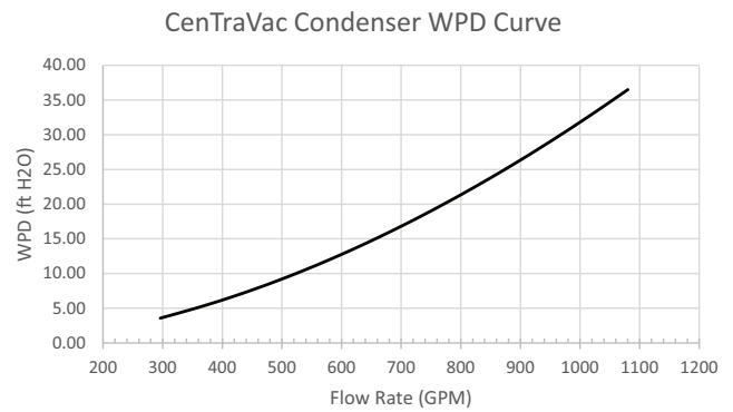
Figure 4. Condenser PD Curve
