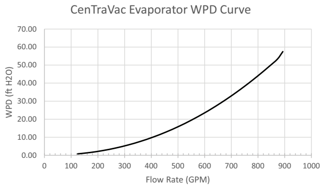
Figure 1. Evaporator PD Curve
