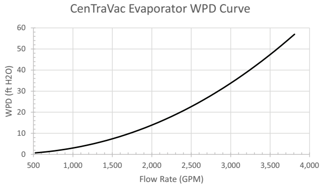
Figure 47. Evaporator PD Curve
