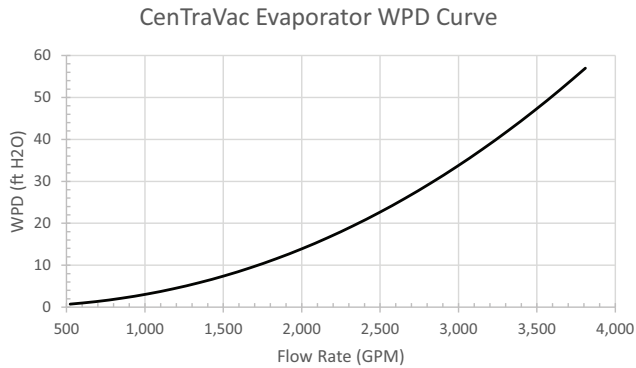
Figure 49. Evaporator PD Curve
