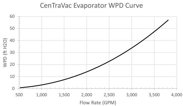
Figure 39. Evaporator PD Curve
