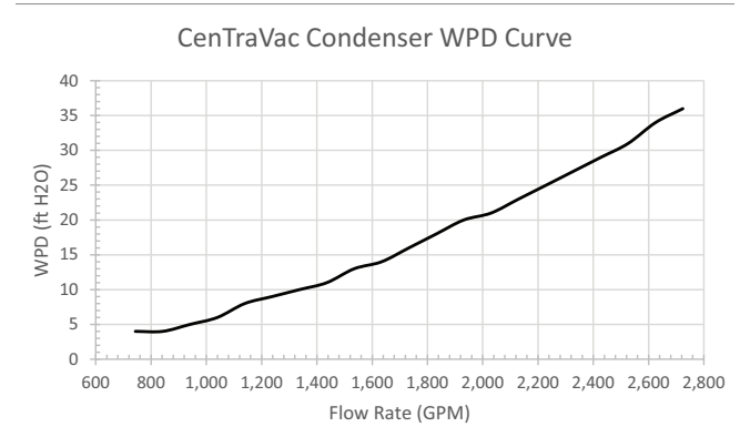
Figure 30. Condenser PD Curve
