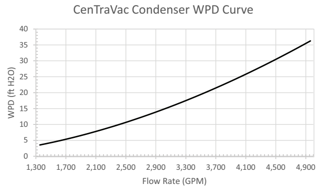
Figure 44. Condenser PD Curve
