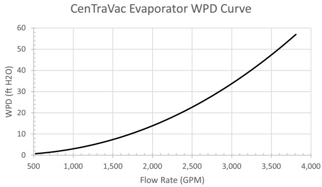
Figure 33. Evaporator PD Curve
