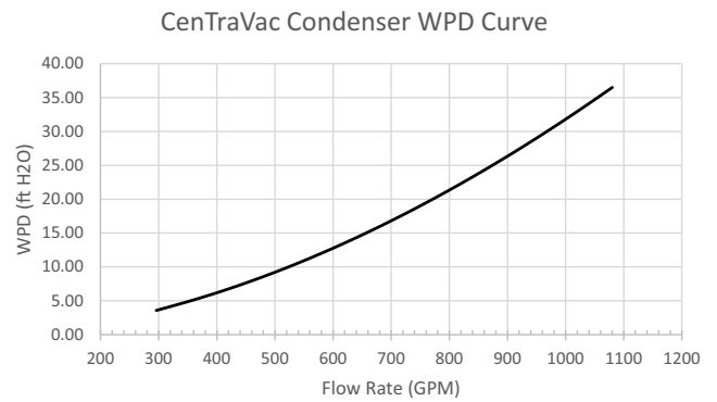
Figure 6. Condenser PD Curve
