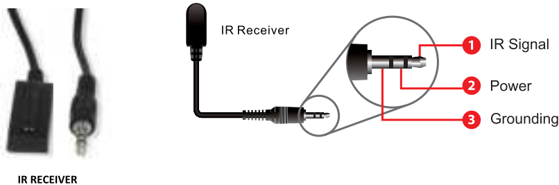
IR RECEIVER
