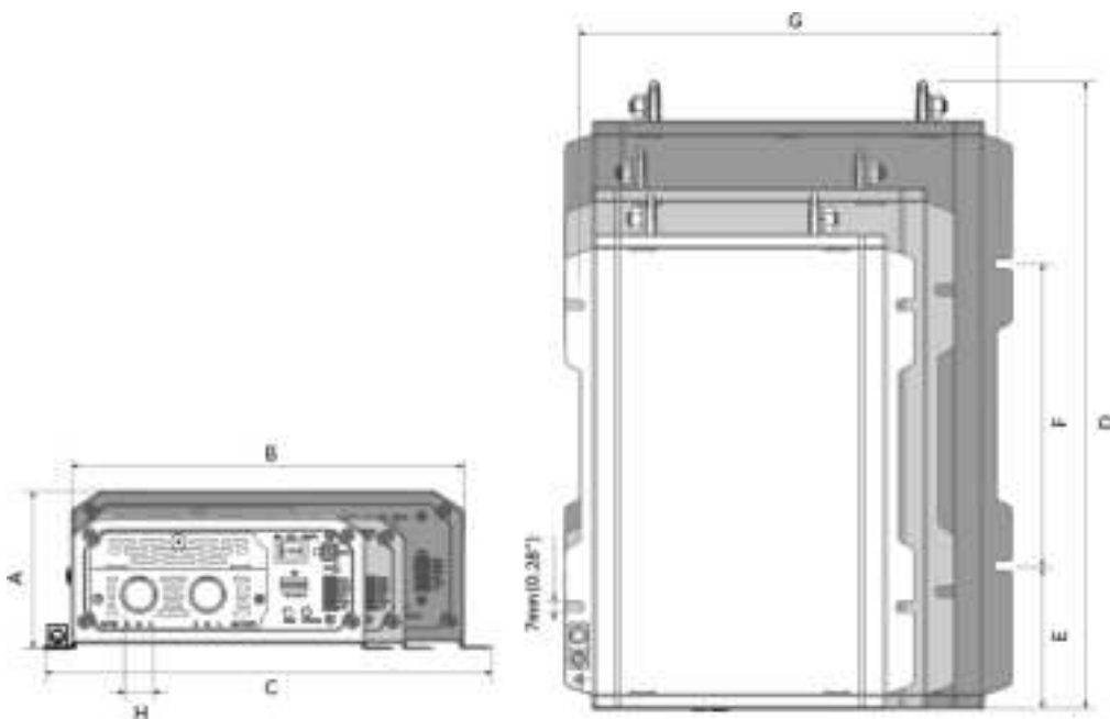
Figure 3. SPT series drawing
