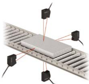
Measuring the thickness/width of a steel plate
