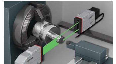
Measuring the run-out of a rotating shaft
