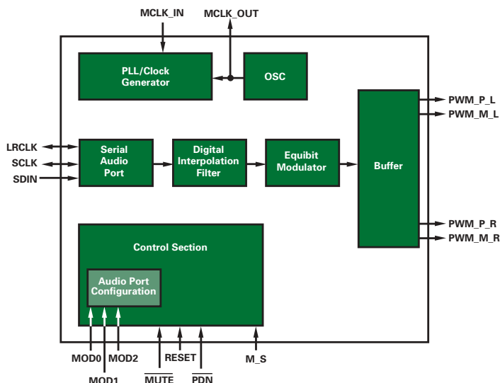
TAS50xx Block Diagram
