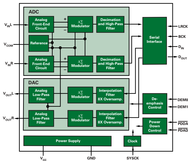
PCM3008 Block Diagram
