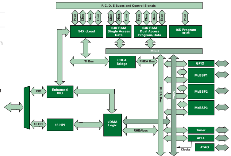
TMS320DA150 Block Diagram
