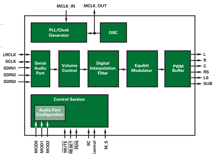
TAS5026/36 Block Diagram
