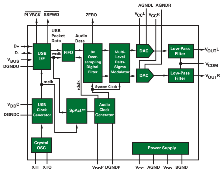
PCM2702 Block Diagram
