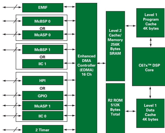
TMS320DA61x Floating-Point DSP Block Diagram
