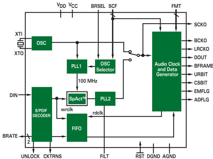
DIR1703 Block Diagram
