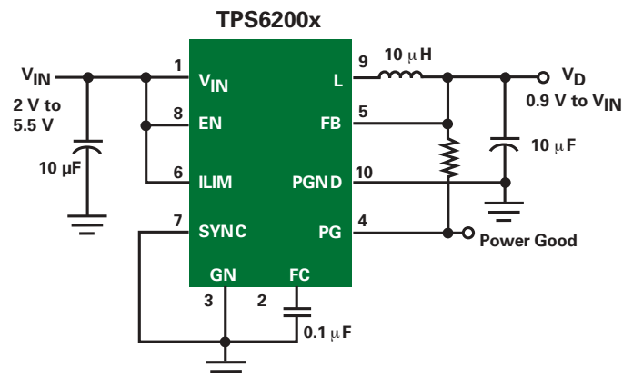
TPS6200x Block Diagram
