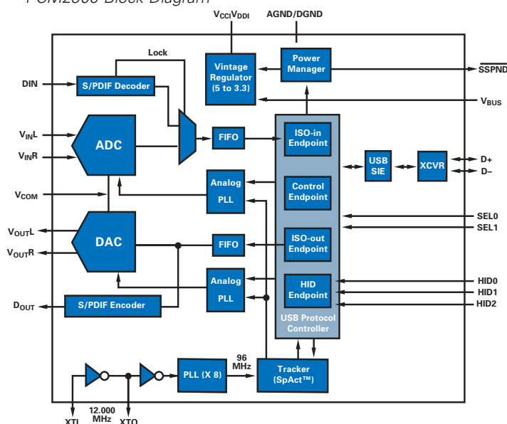
PCM2900 Block Diagram
