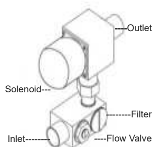
1. Solenoid Valve
