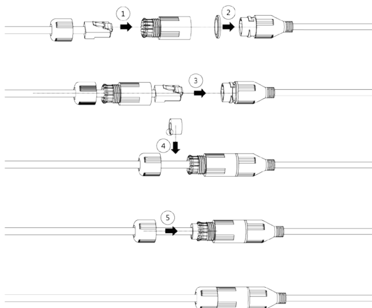
Figure 3-7 Install waterproof connector
