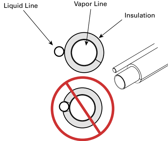
Figure 5. Refrigerant line insulation
