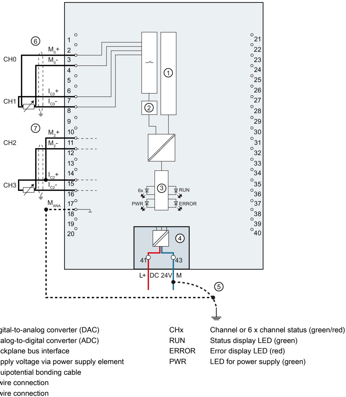
Figure 3-6 Block diagram and pin assignment for 3- and 4-wire connection
