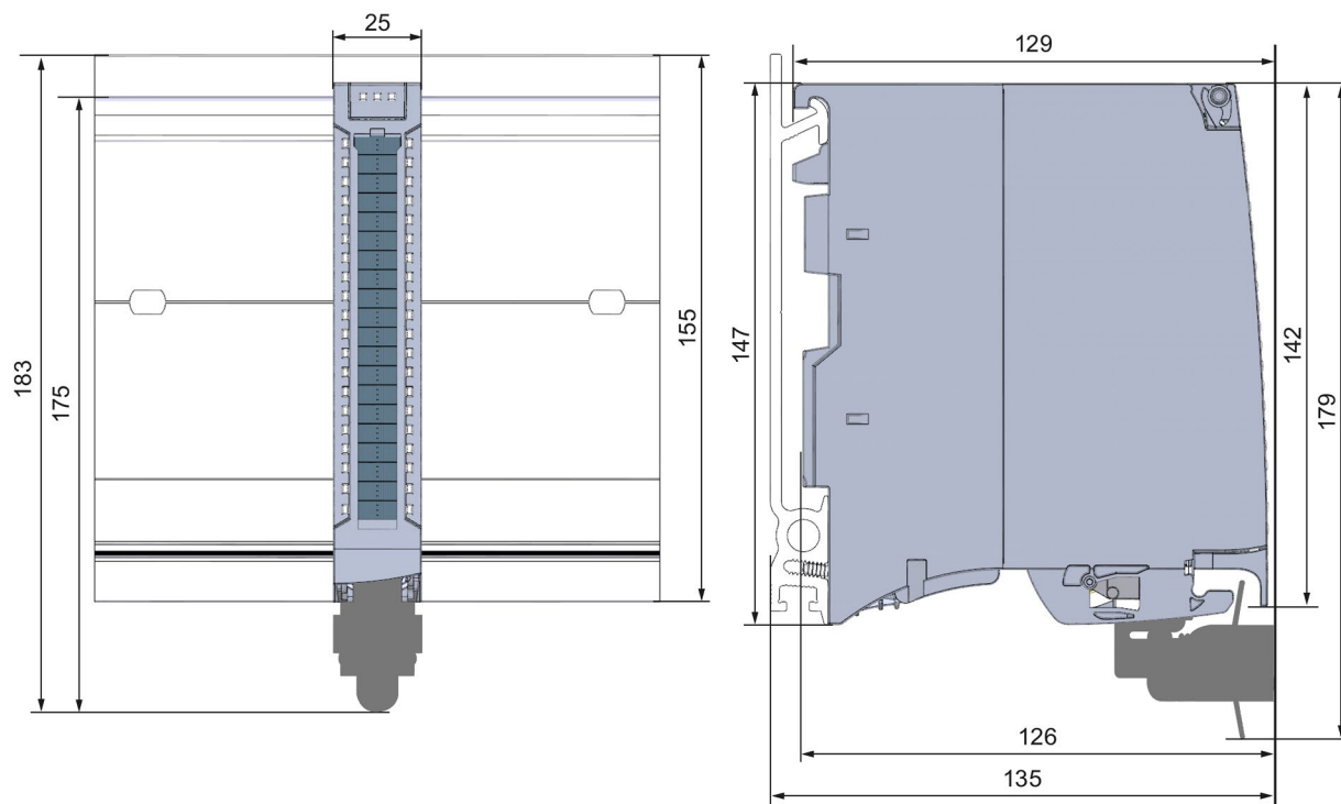
Figure A-1 Dimension drawing of the AI 4xU/I/RTD/TC/ AQ 2xU/I ST module
