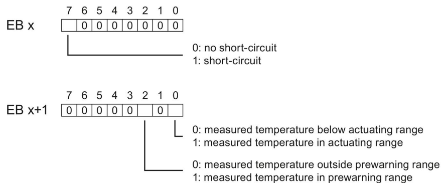
Figure 4-1 Address space for AI 4xU/I/RTD/TC/ AQ 2xU/I ST with PTC resistors
