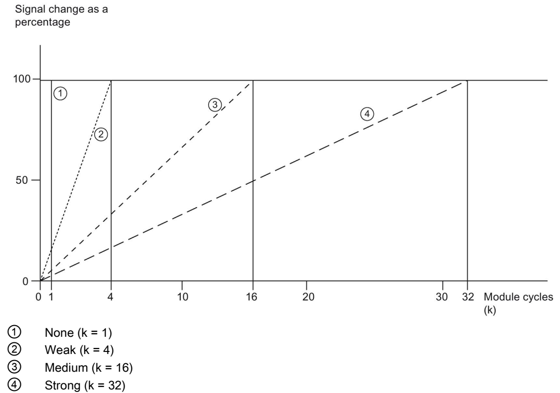
Figure 4-3 Smoothing with AI 4xU/I/RTD/TC/ AQ 2xU/I ST
