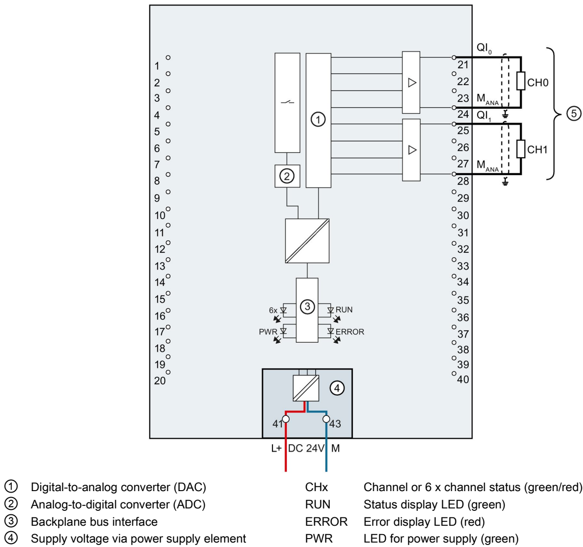
Figure 3-10 Block diagram and pin assignment for the current output
