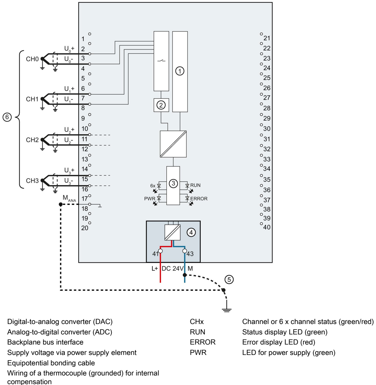
Figure 3-8 Block diagram and pin assignment for grounded thermocouples
