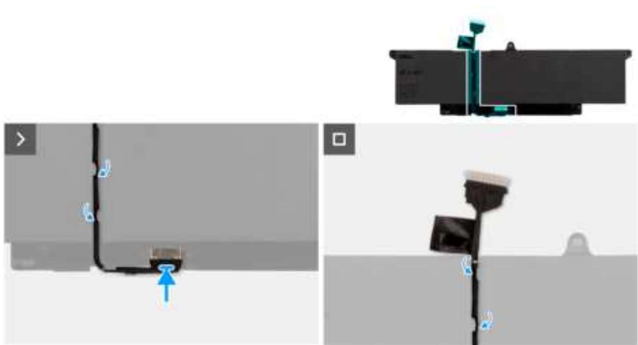
Figure 23. Installing the battery cable
