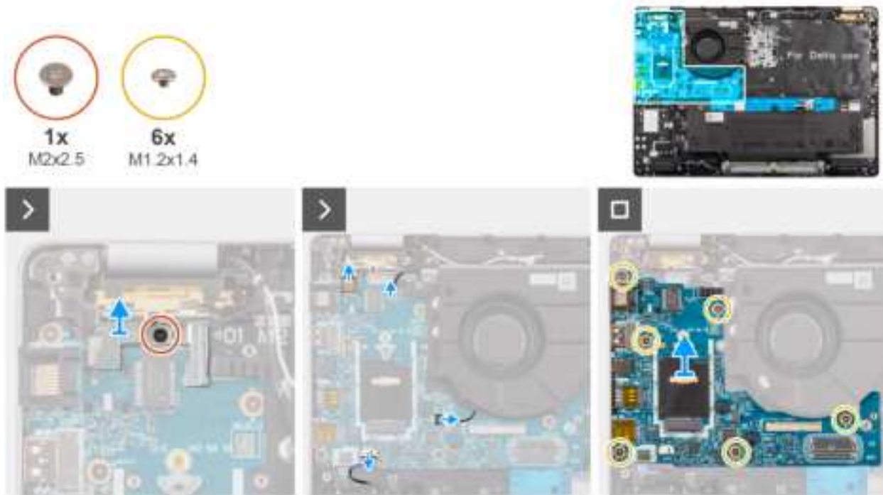
Figure 46. Removing the I/O board
