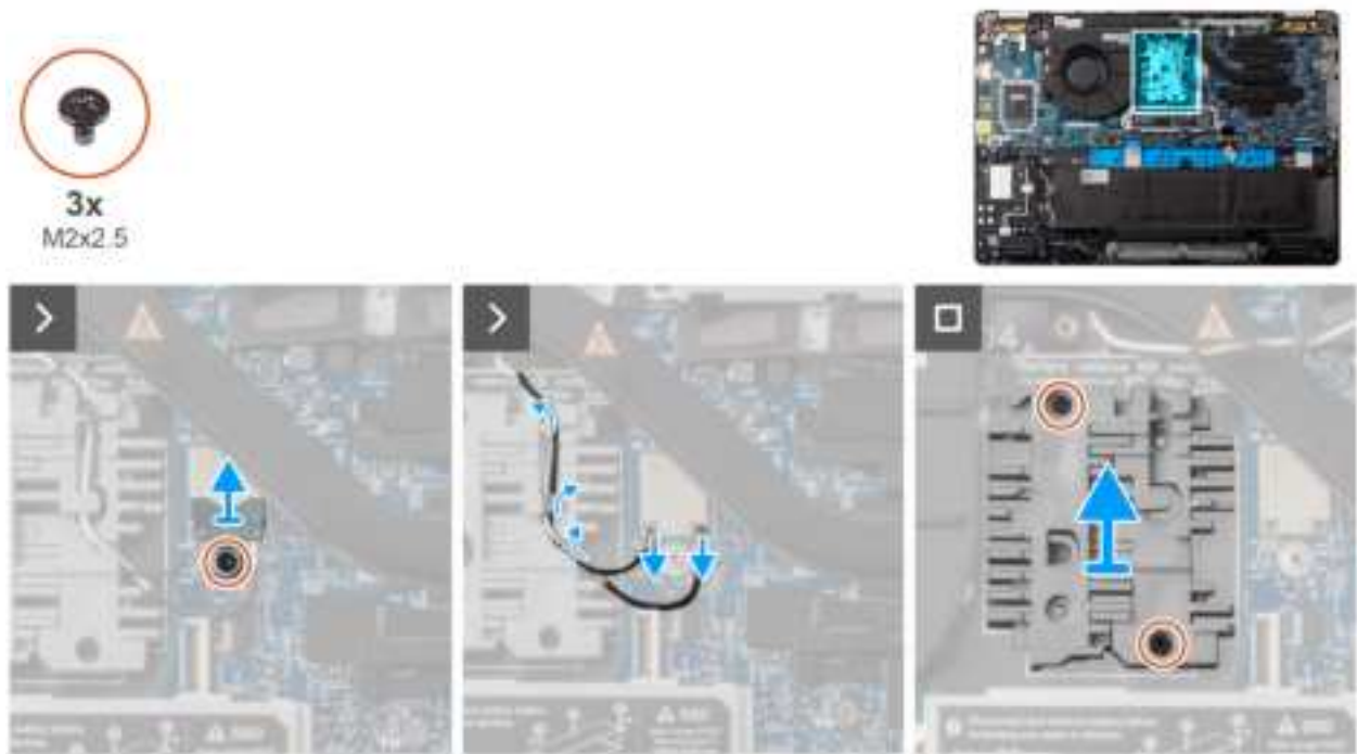
Figure 81. Removing the keyboard filler
