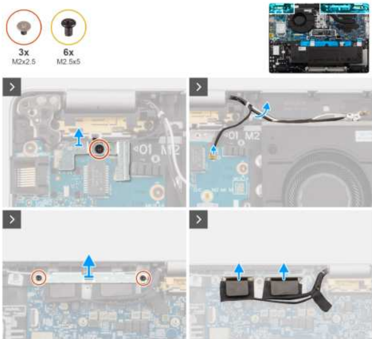
Figure 52. Removing the display assembly
