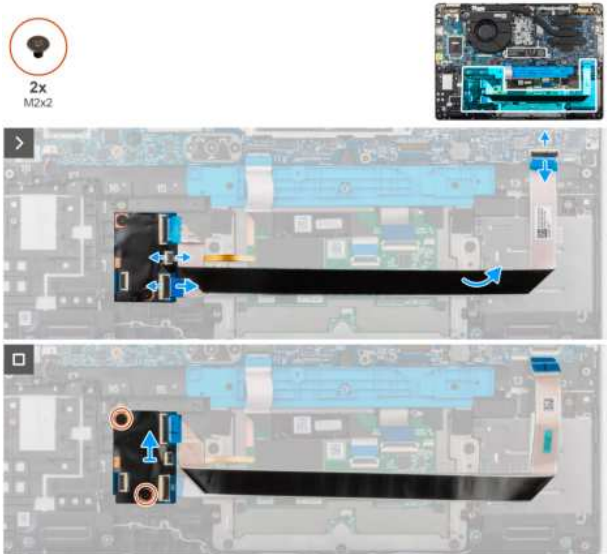
Figure 34. Removing the USH board
