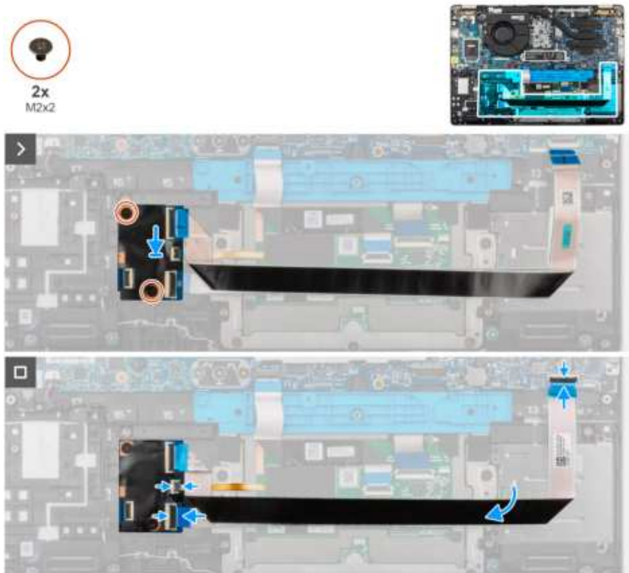
Figure 35. Installing the USH board
