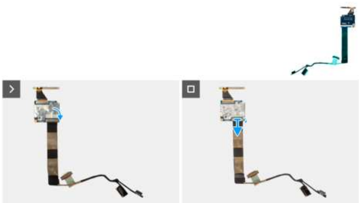
Figure 70. Removing the display cable
