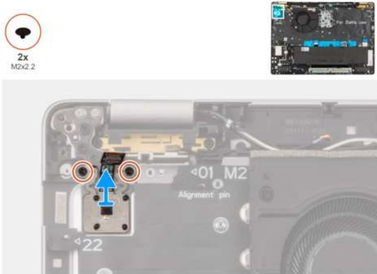
Figure 50. Removing the power button with optional fingerprint reader
