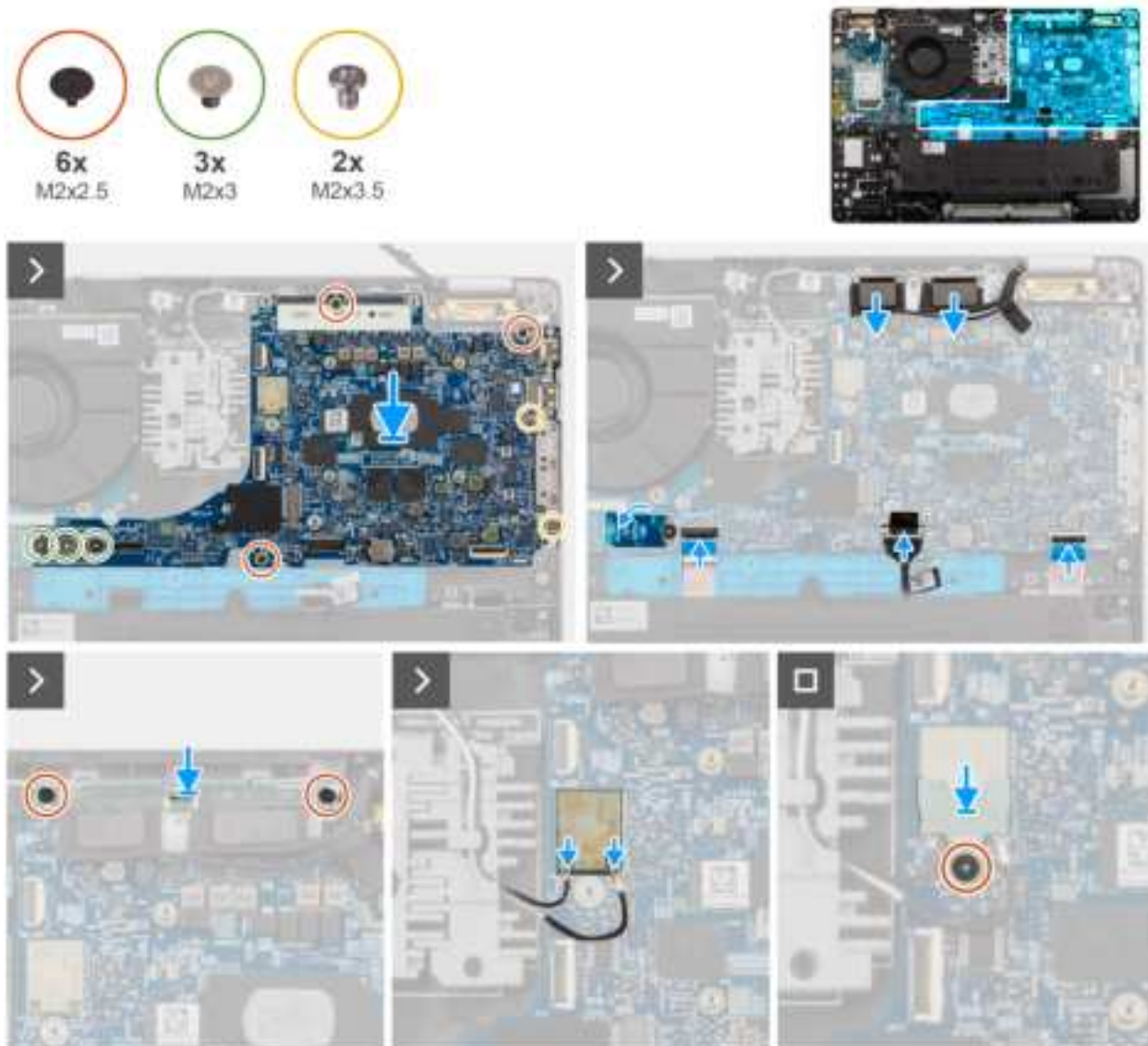
Figure 45. Installing the system board
