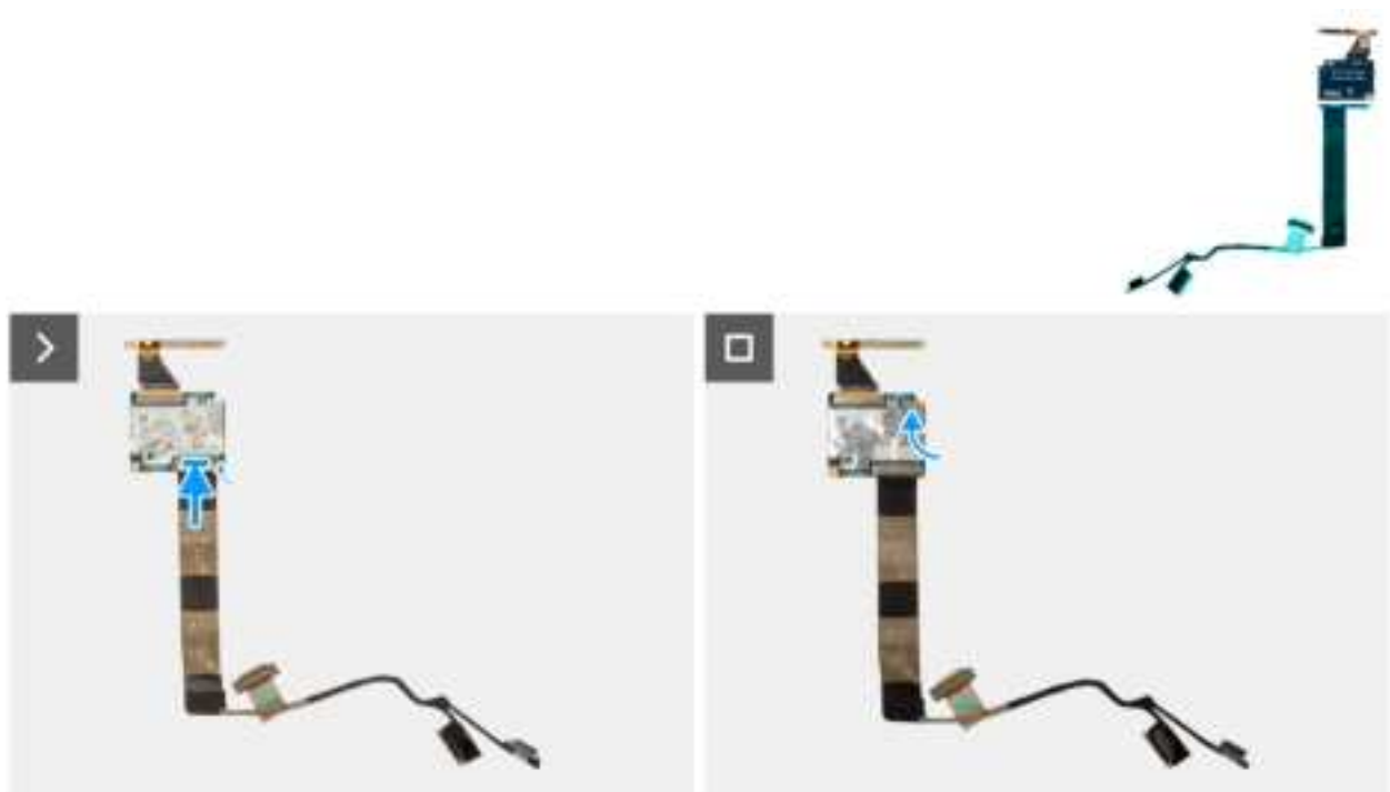
Figure 71. Installing the display cable
