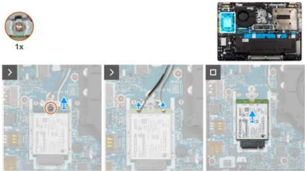
Figure 28. Removing the 4G WWAN card
