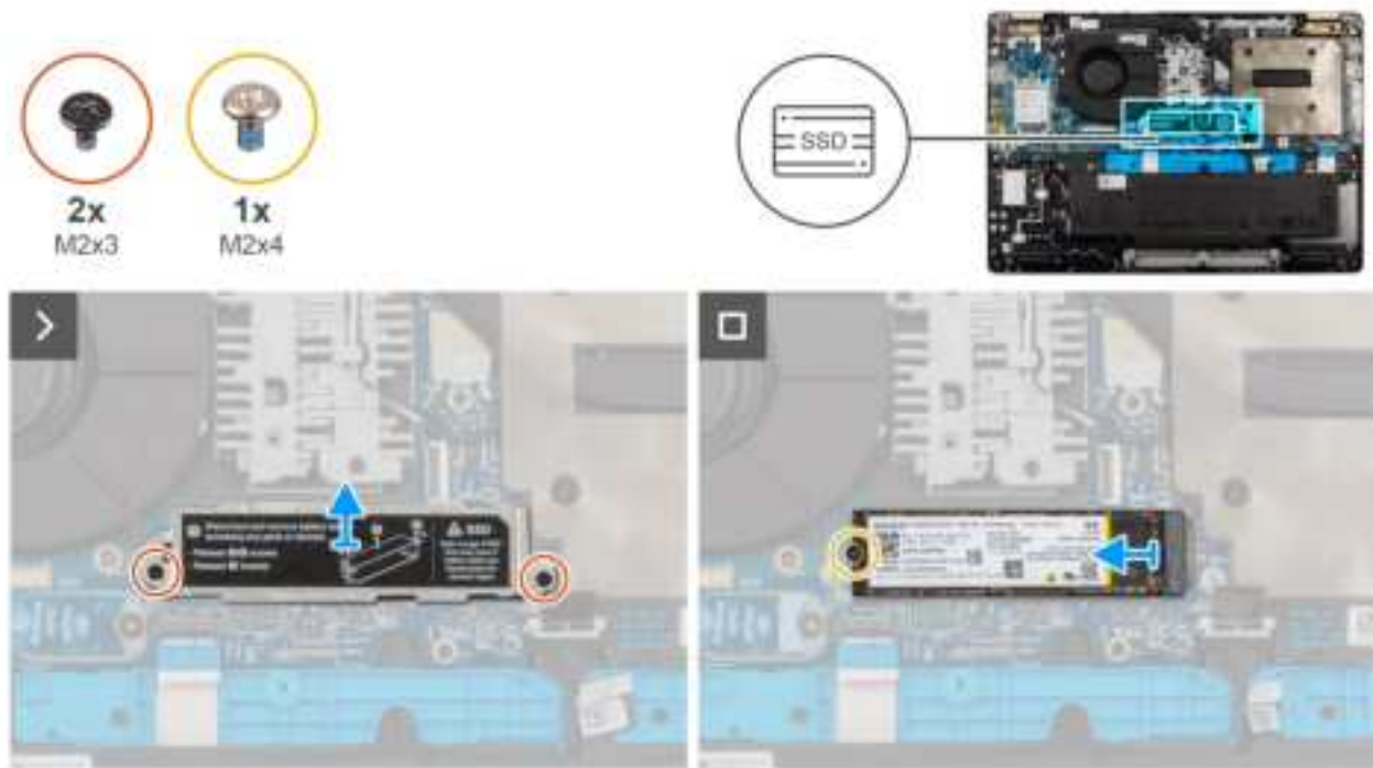
Figure 26. Removing the M.2 2280 SSD
