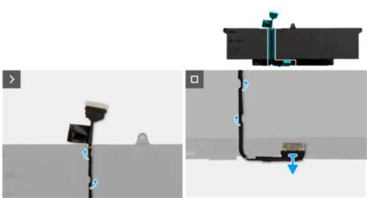
Figure 22. Removing the battery cable
