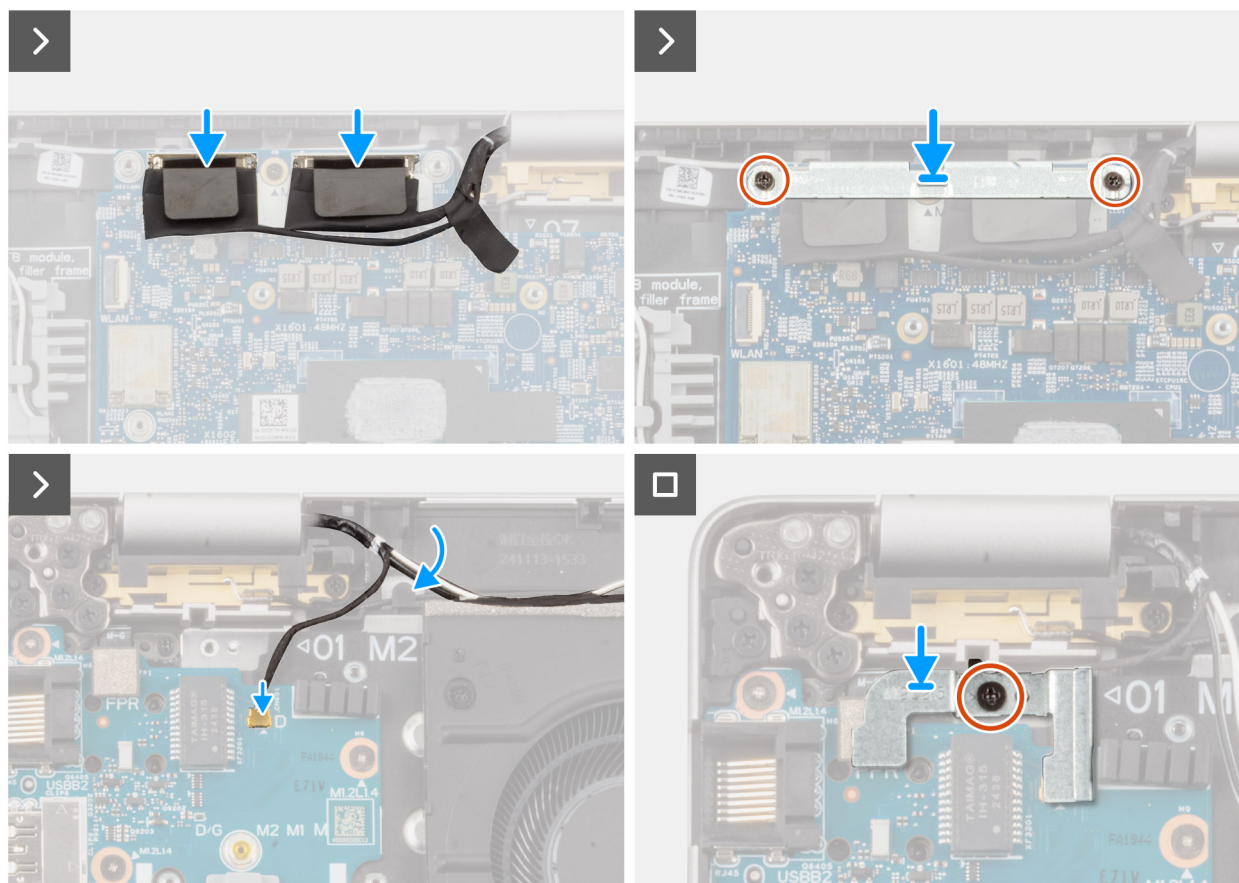
Figure 55. Installing the display assembly
