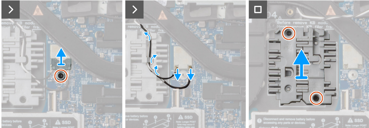
Figure 81. Removing the keyboard filler
