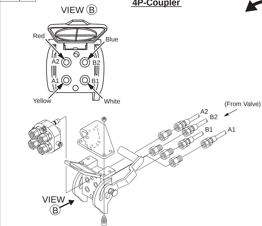
Coupler
