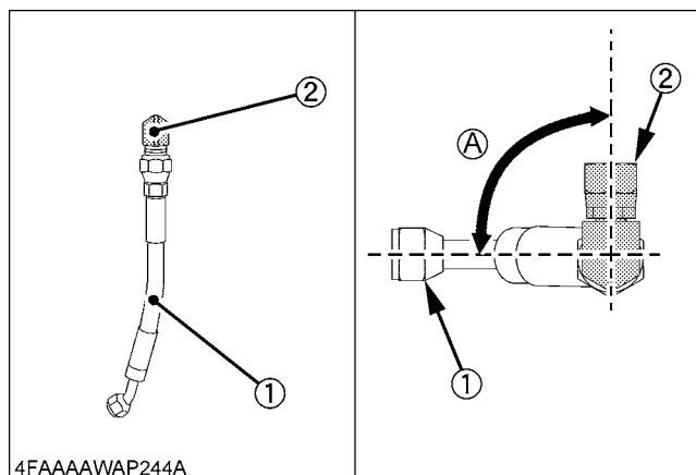
4FAAAAWAP244A (1) Pilot tank line hose (230 mm (9.1 in.), 3/4-UNF) (A) 90° (2) Elbow adapter (3/4-UNF)
