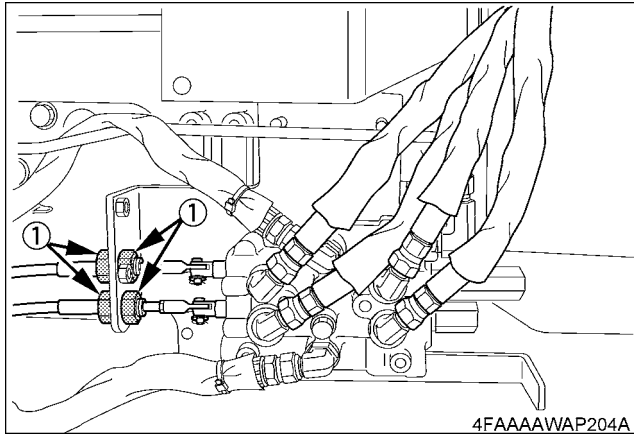
(1) 4-M16 lock nuts
