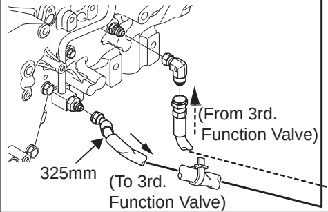
Tractor's Hydraulic Power for Pilot Take-off (T.H.P.P.T.)
