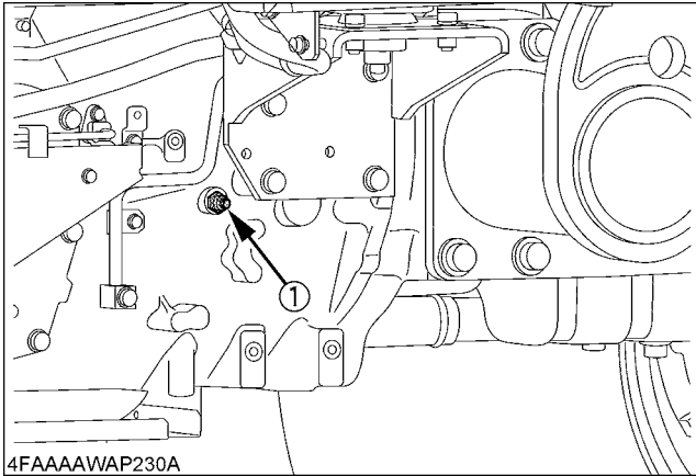
(1) Adapter (1/4-BSPT)
