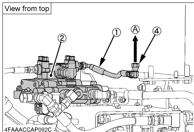
4FAAACCAP092C (1) Pilot tank line hose (230 mm (9.1 in.), 9/16-UNF) (A) Connect to the pilot tank port of the tractor (2) 3rd function valve (3) Pilot tank port of the tractor (4) Elbow adapter (9/16-UNF)
