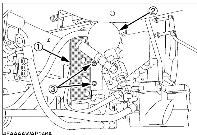
(1) Stay (2) Accumulator assy (3) 2-M8 x 25 bolts with washer
