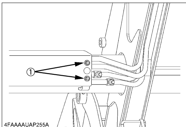
(1) 2-M8 x 35 bolts with washers
