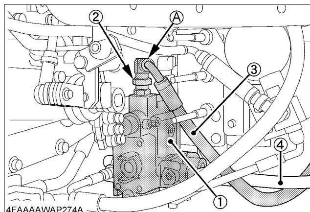
4FAAAAWAP274A (1) 3rd function valve (A) 90° side (2) Port A (3) Port A hose (Gray: 1340 mm (52.8 in.), 3/4-UNF) (4) Pump line hose
