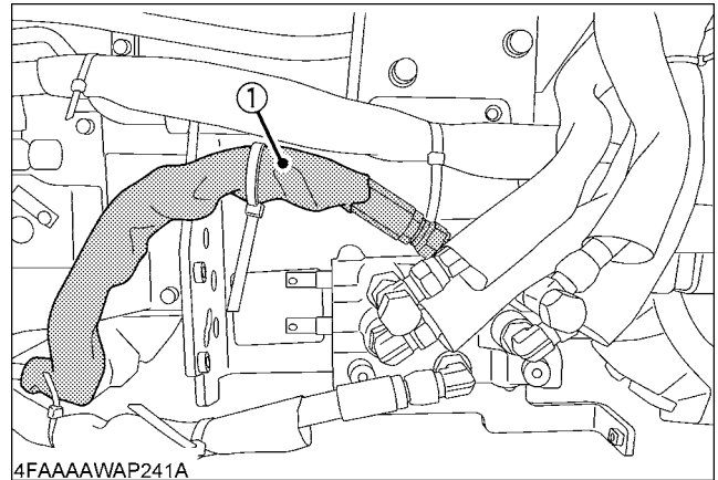
(1) Pump line hose (630 mm (24.8 in.))
