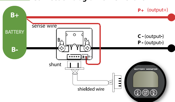
Figure 3 Connection diagram of 75A shunt
