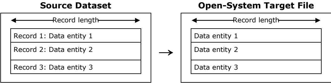
Figure 2-9 FXmto with Fixed-Length Records: No Padding, No Delimiters
