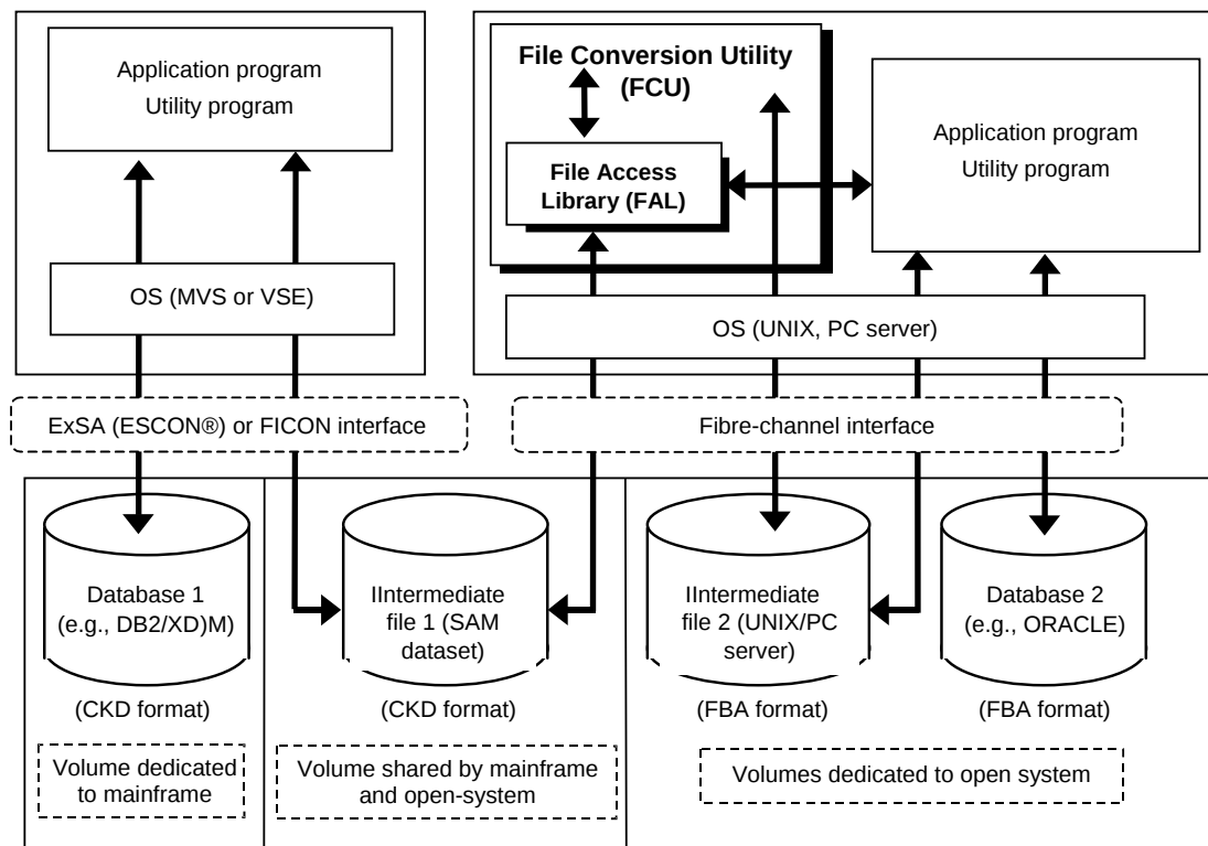
Figure 2-1 FXmto and FXotm System Configuration
