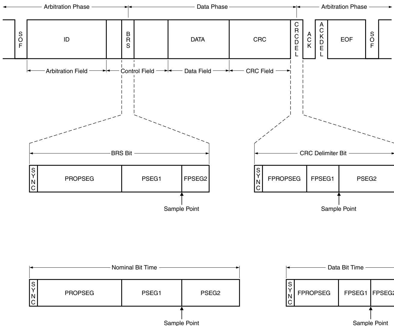
Figure 49-3. Bit rate switching mechanism for CAN FD messages
