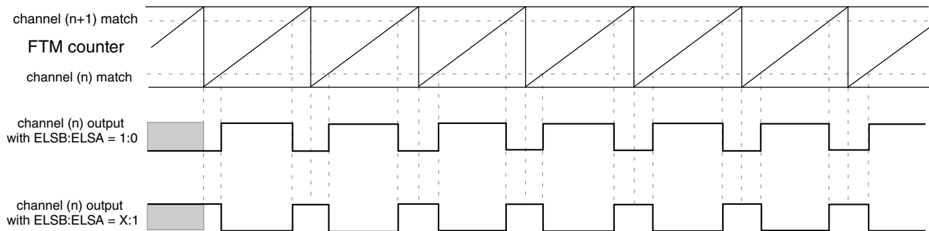
Figure 41-30. Combine mode
