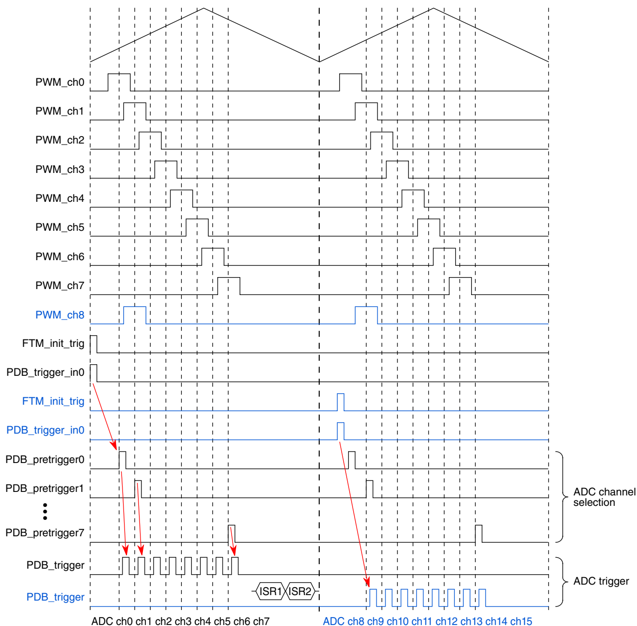
Figure 37-15. Example: PWM Load Diagnosis – ADC Trigger Concept 2 (Timing)
