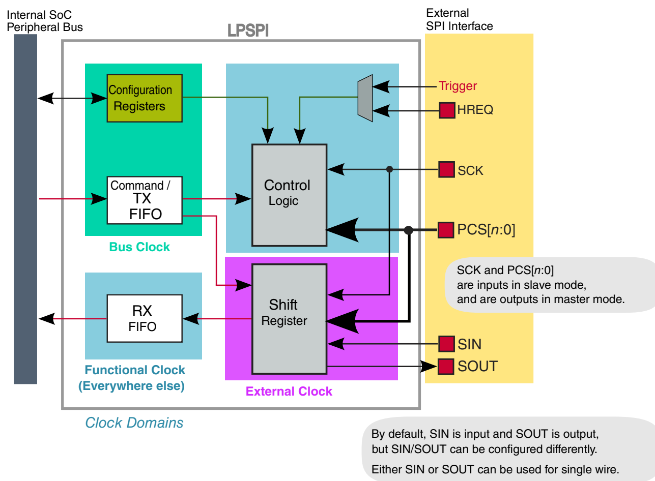
Figure 45-1. Block Diagram
