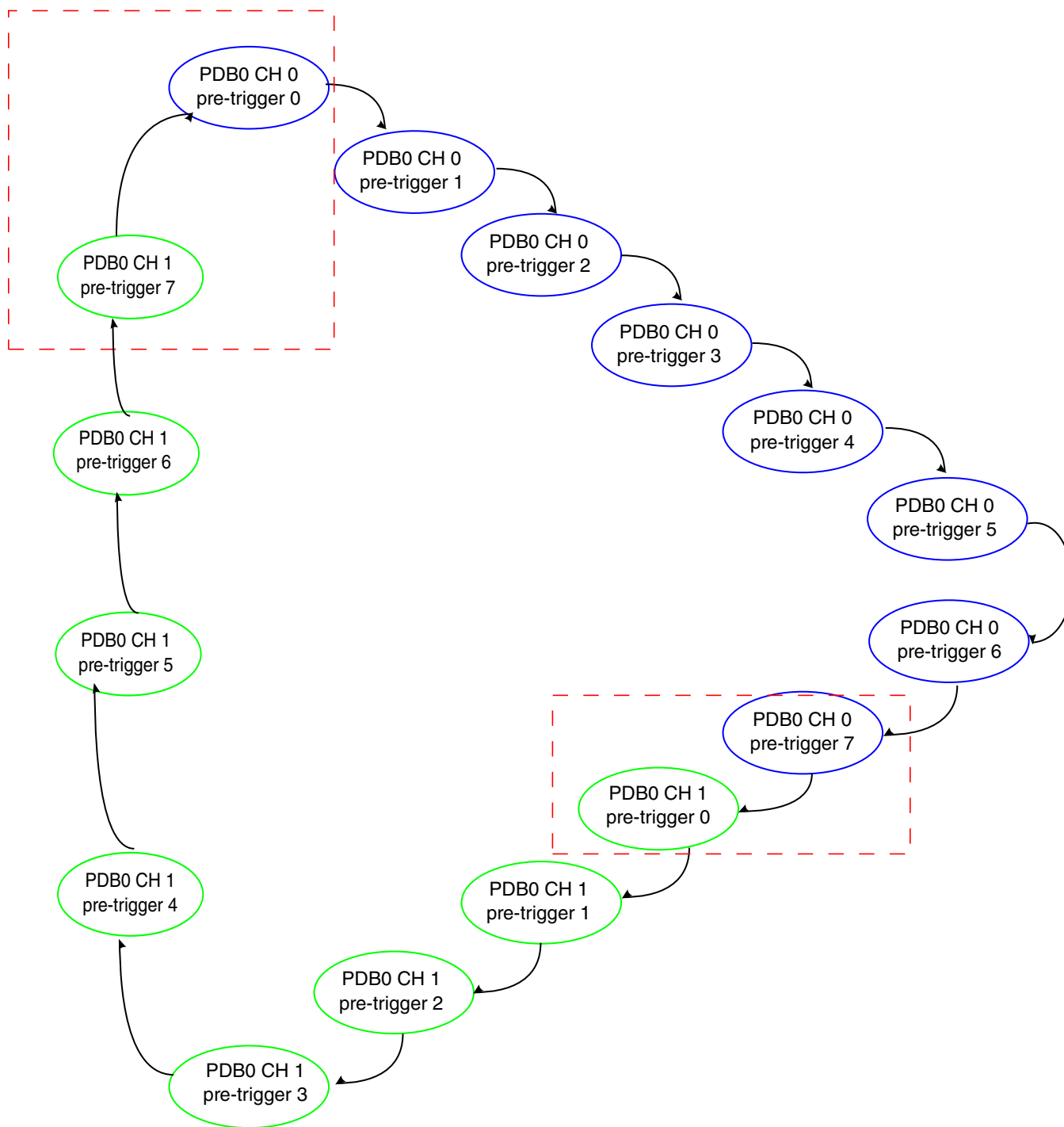
Figure 40-4. PDB back-to-back chain forming PDB0-PDB1 ring
