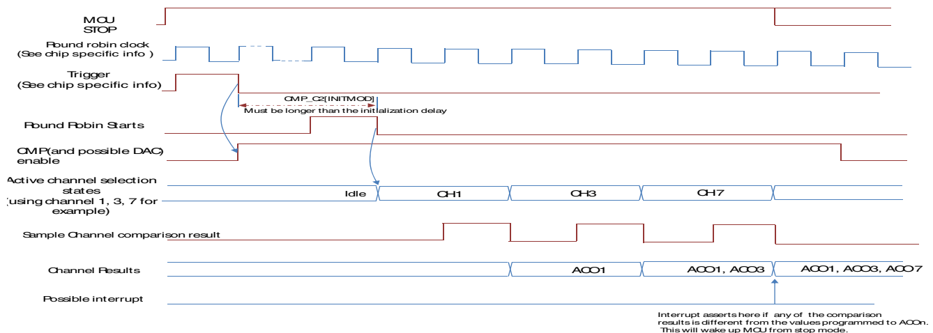
Figure 39-16. Trigger mode
