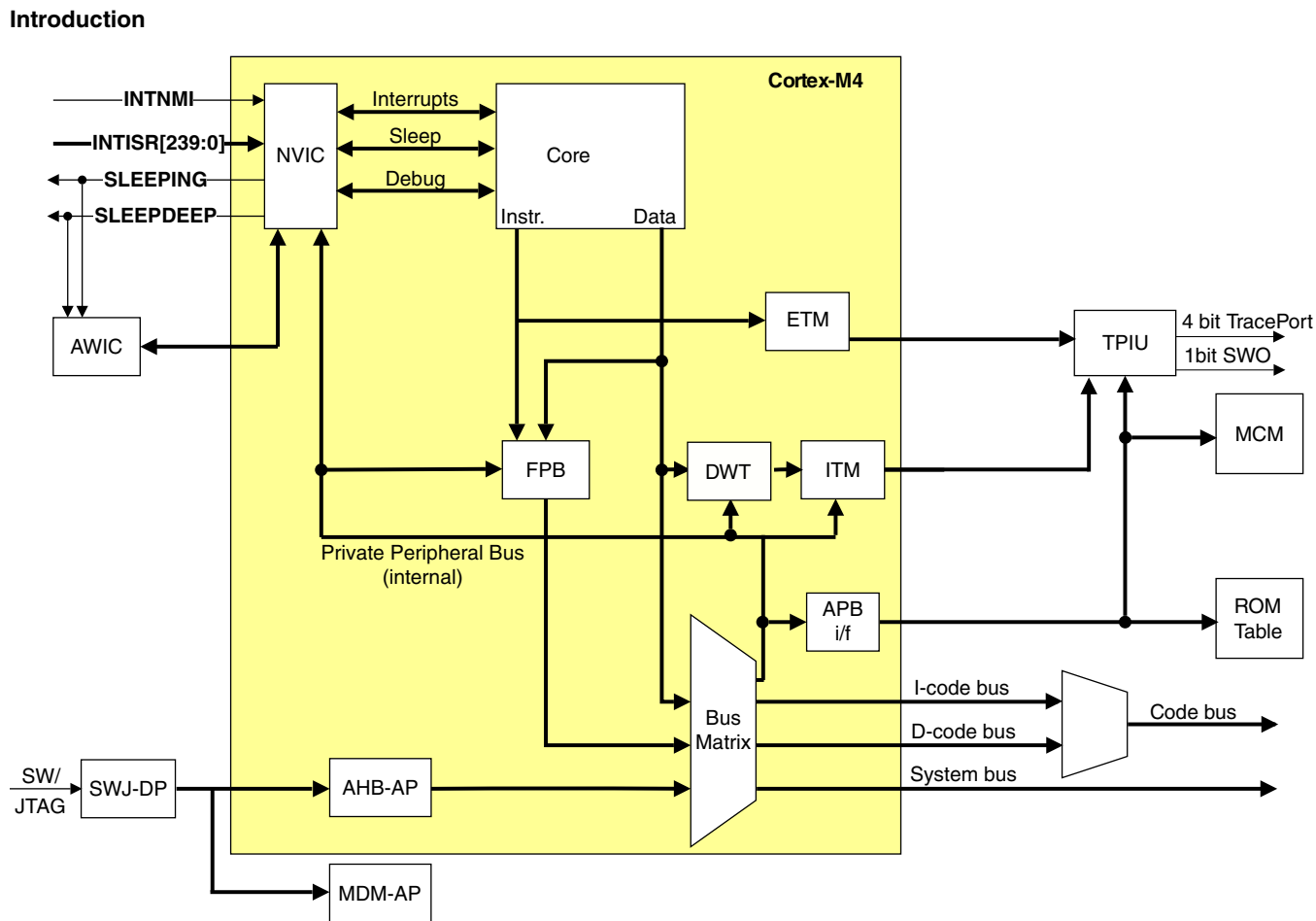
Figure 52-1. Cortex-M4 debug topology
