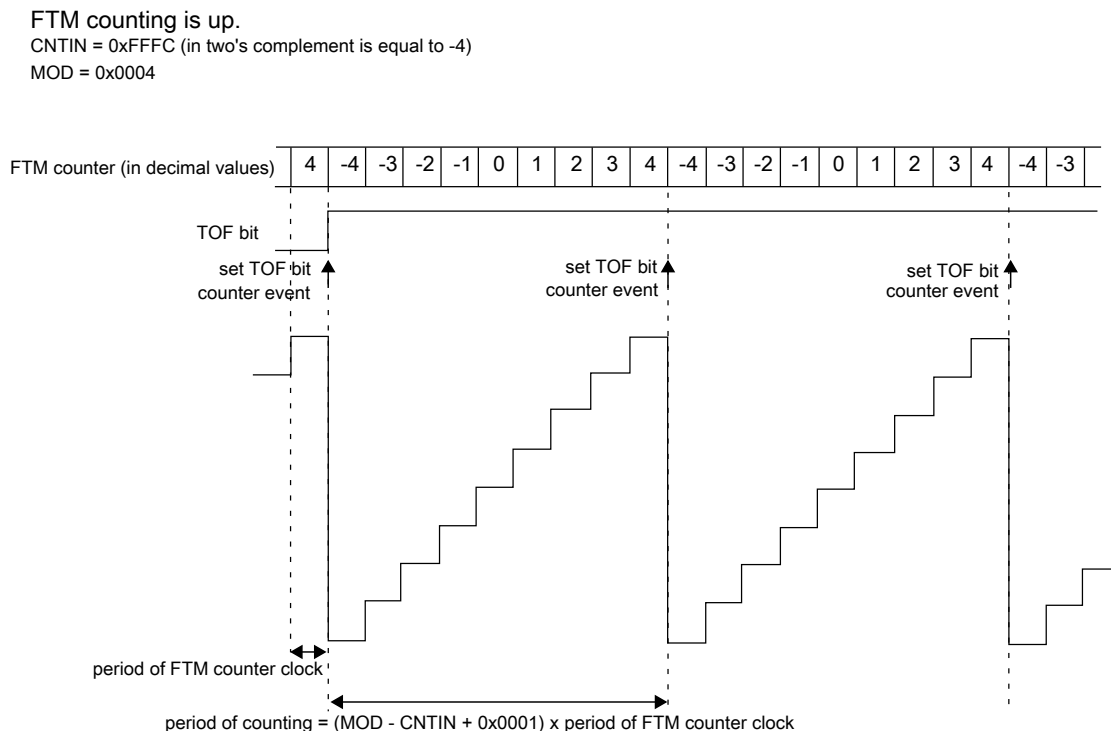
Figure 41-8. Example of FTM up and signed counting
