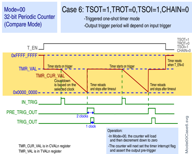
Figure 42-10. Case 6: TSOT = 1, TROT = 0, TSOI = 1, CHAIN = 0
