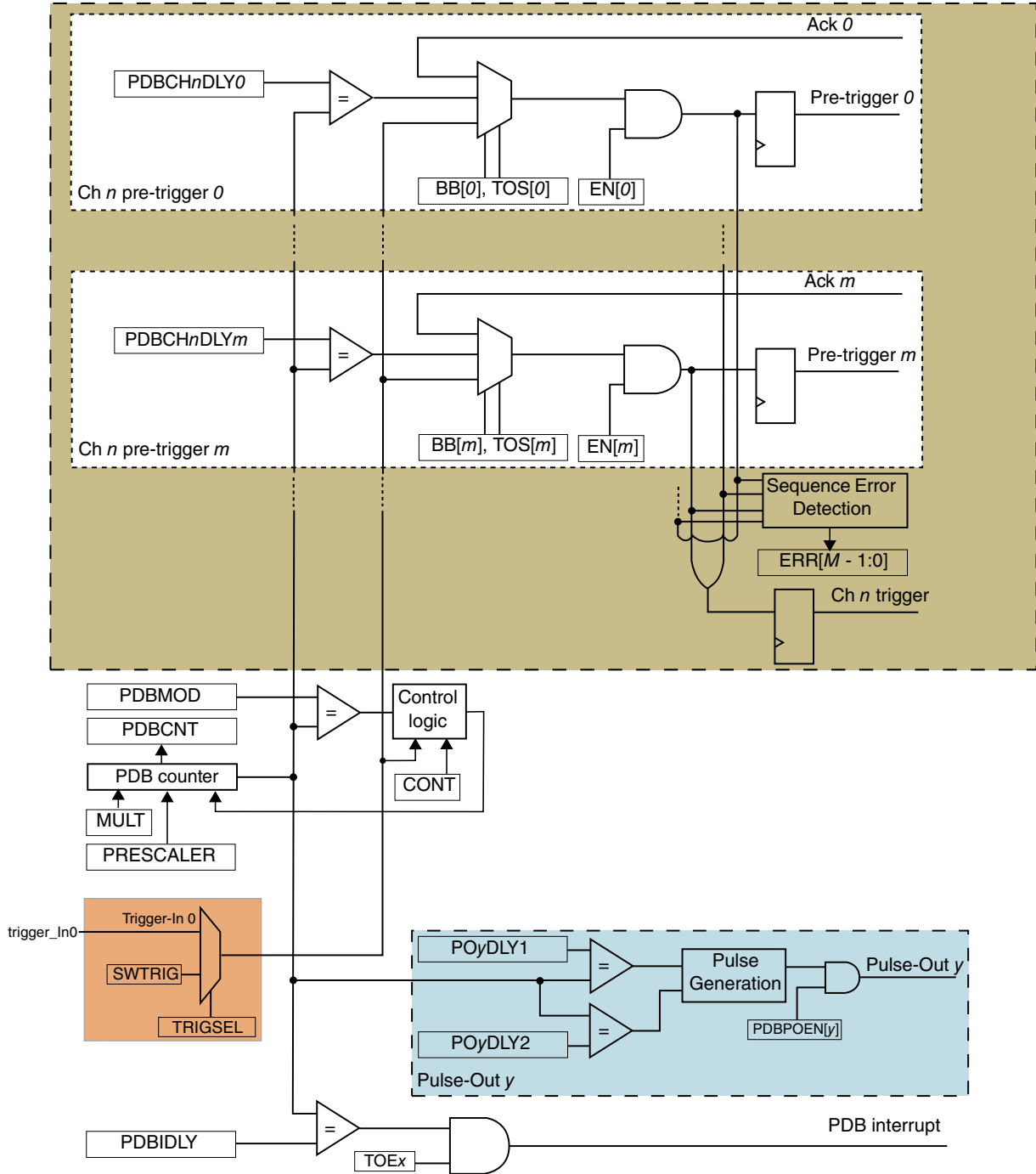
Figure 40-7. PDB block diagram
