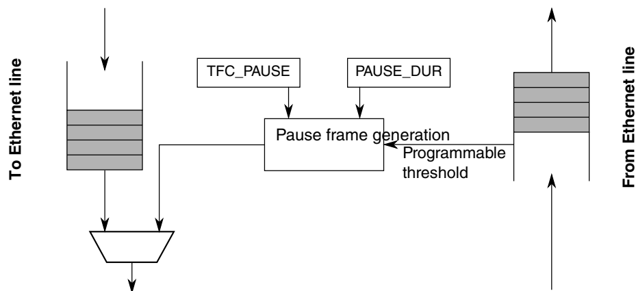
Figure 51-8. Pause frame generation overview
