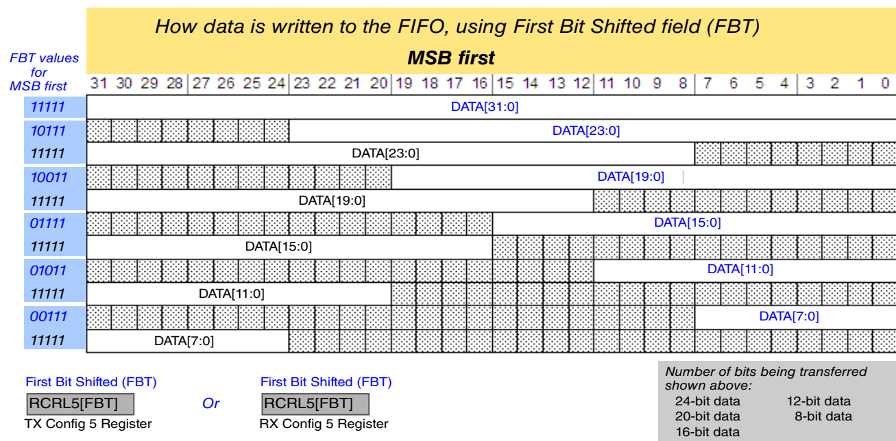
Figure 50-4. SAI first bit shifted, MSB first
