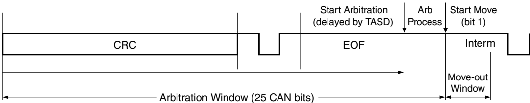
Figure 49-10. Arbitration and move-out time windows
