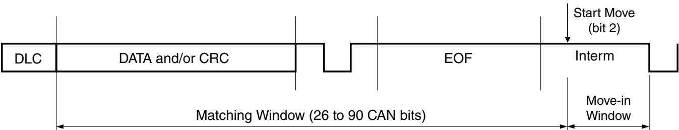
Figure 49-9. Matching and move-in time windows
