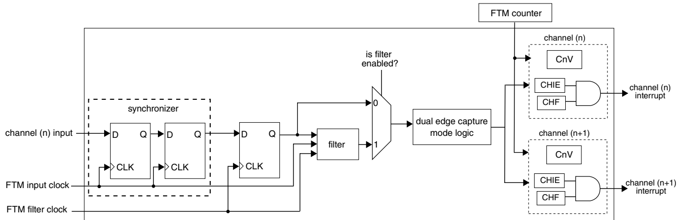
Figure 41-95. Diagram for Dual Edge Capture Mode when FLTPS[3:0] ≠ 0
