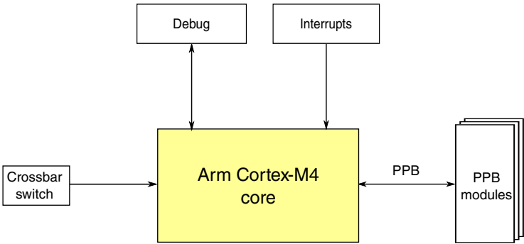
Figure 7-1. Core configuration
