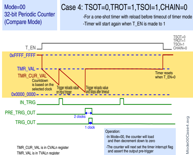
Figure 42-8. Case 4: TSOT = 0, TROT = 1, TSOI = 1, CHAIN = 0
