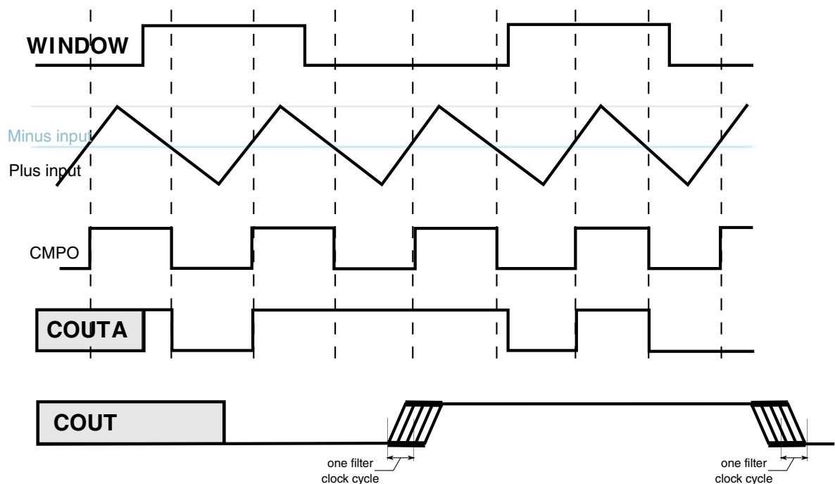
Figure 39-14. Windowed/Filtered mode operation
