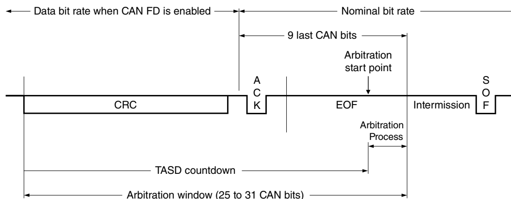
Figure 49-12. Optimal Tx Arbitration start point
