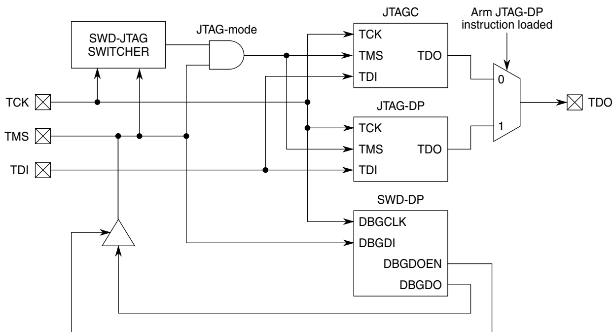
Figure 52-2. Modified debug port
