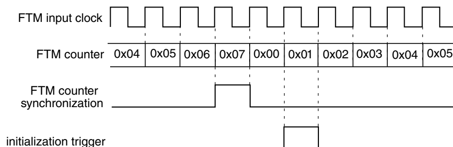
Figure 41-90. Example of the generation of the initialization trigger in the case 3.
