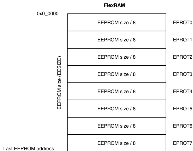
Figure 32-8. EEPROM protection
