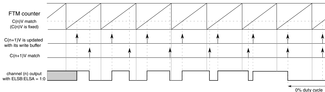
Figure 41-48. Modified Combine PWM Mode Examples
