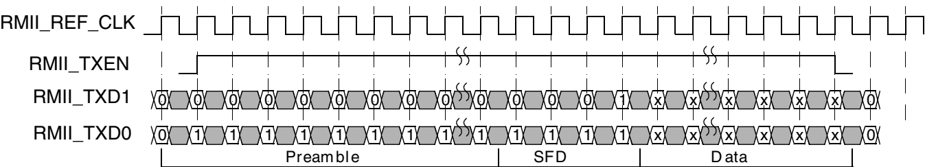
Figure 51-21. RMII transmit operation
