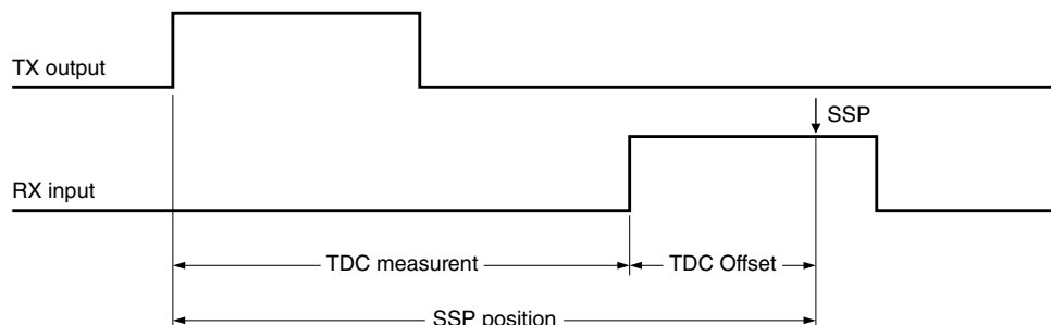
Figure 49-5. SSP position with optimal values
