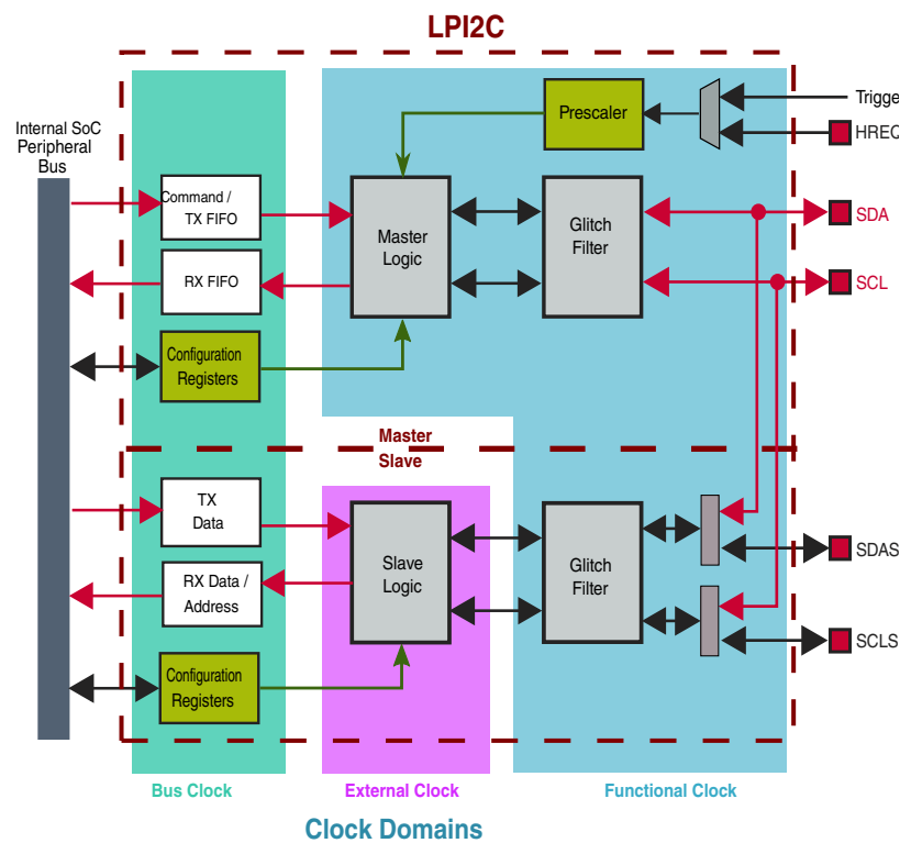
Figure 46-1. LPI2C block diagram
