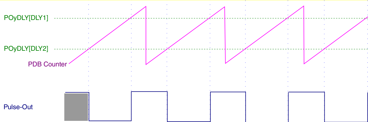
Figure 40-9. How Pulse Out is generated
