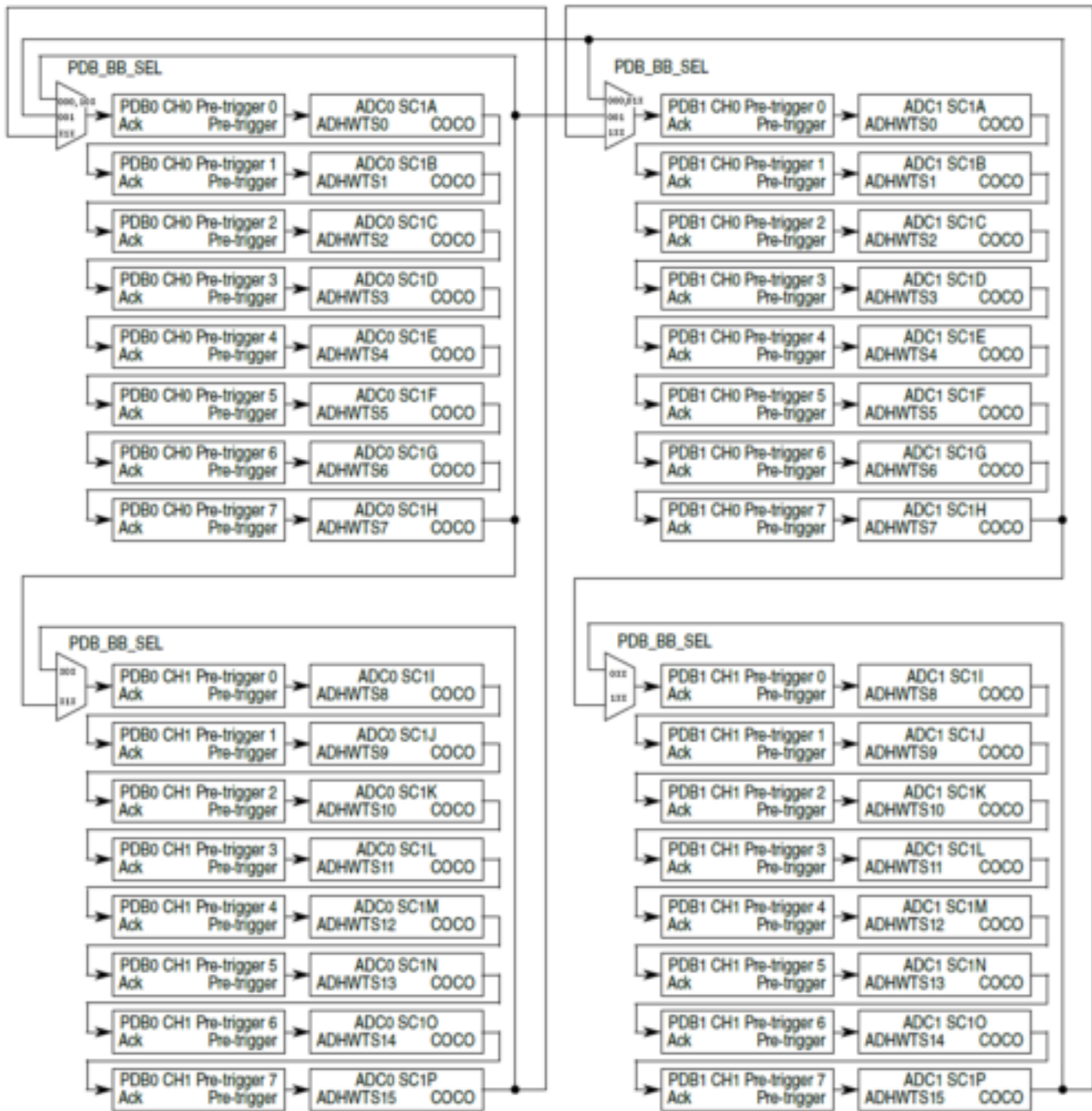
Figure 40-5. PDB-ADC back to back connection (Part 1 of 2)
