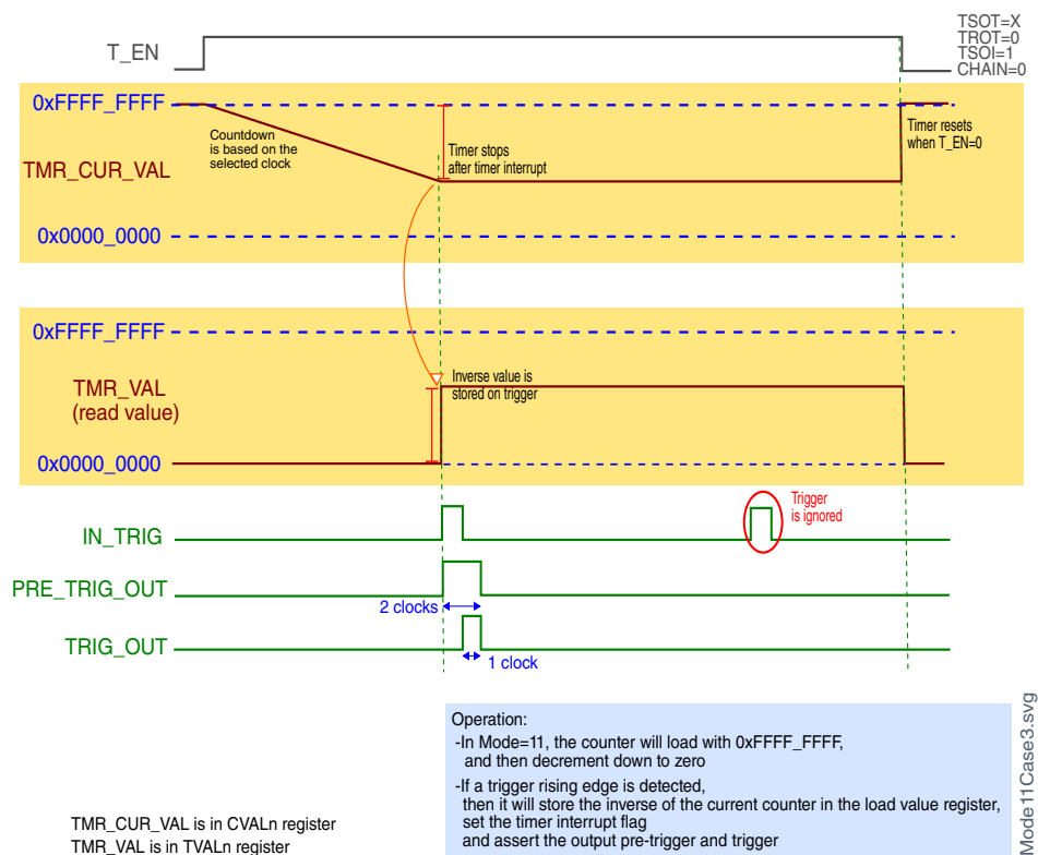
Figure 42-18. Case 3: TSOT = X, TROT = 0, TSOI = 1, CHAIN = 0
