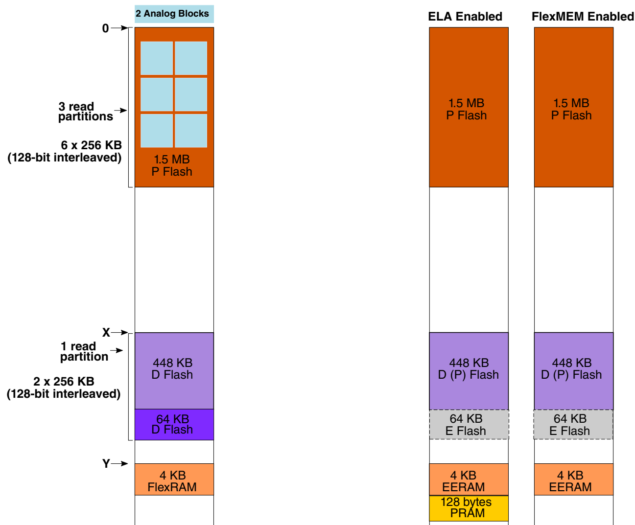
Figure 32-3. 2 MB flash memory map
