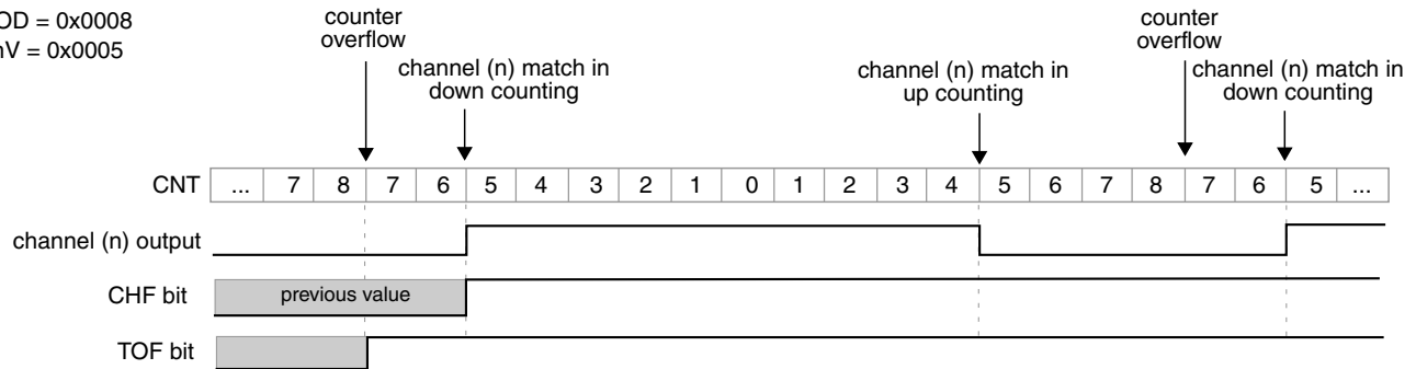
Figure 41-28. CPWM signal with ELSB:ELSA = 1:0
