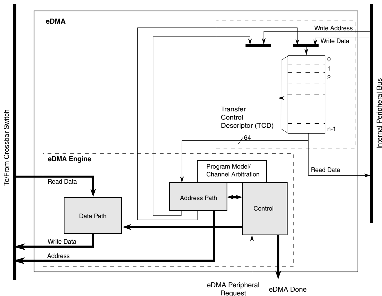
Figure 16-3. eDMA operation, part 2
