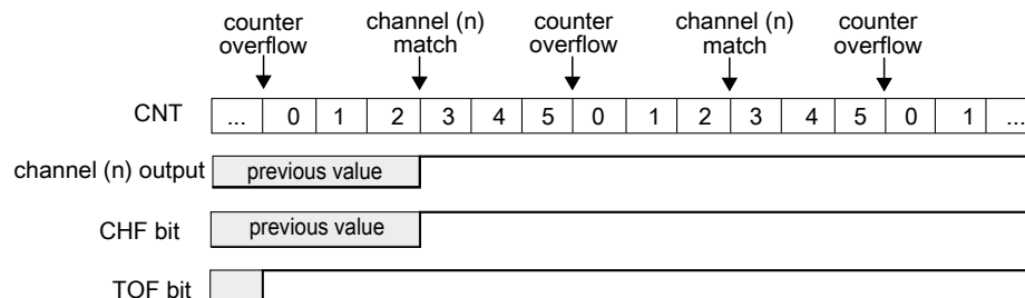
Figure 41-23. Example of the Output Compare mode when the match sets the channel output
