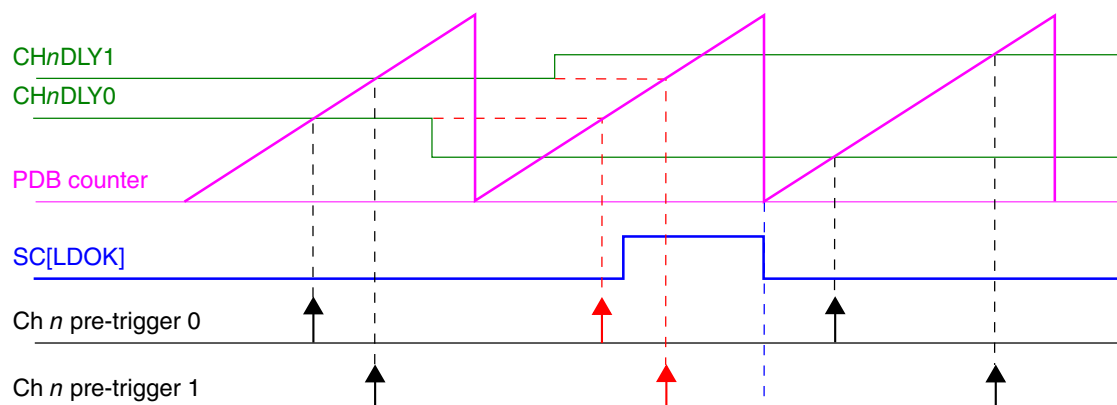
Figure 40-11. Registers update with SC[LDMOD] = x1
