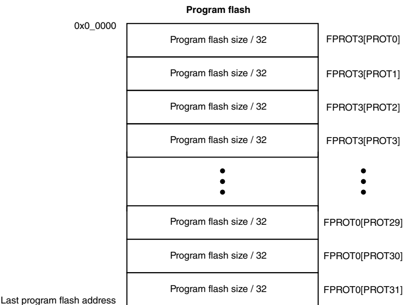
Figure 32-6. Program flash protection
