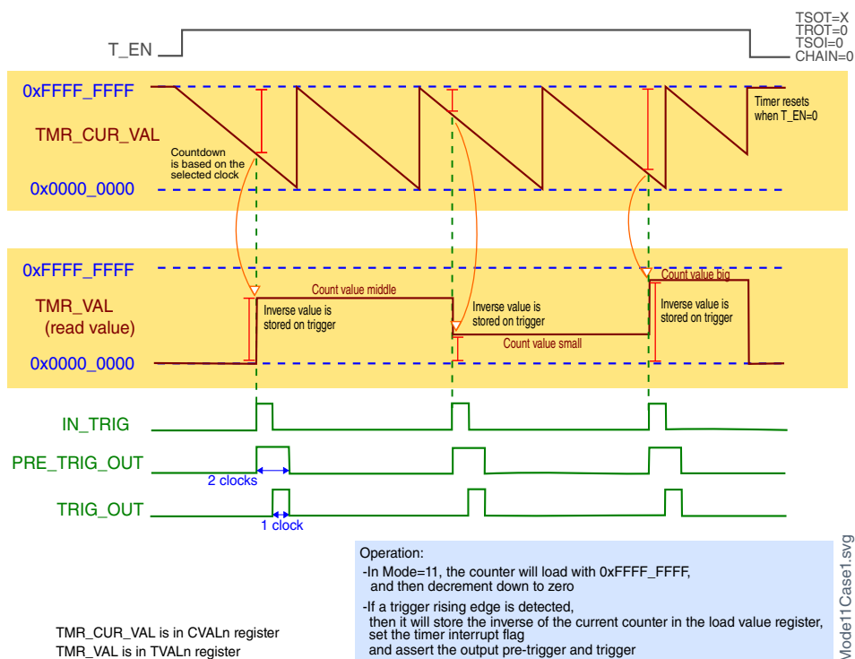
Figure 42-16. Case 1: TSOT = X, TROT = 0, TSOI = 0, CHAIN = 0
