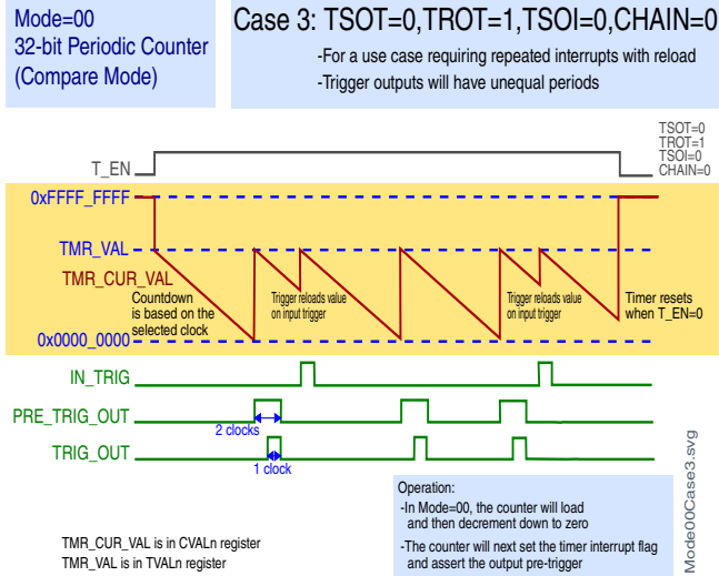
Figure 42-7. Case 3: TSOT = 0, TROT = 1, TSOI = 0, CHAIN = 0
