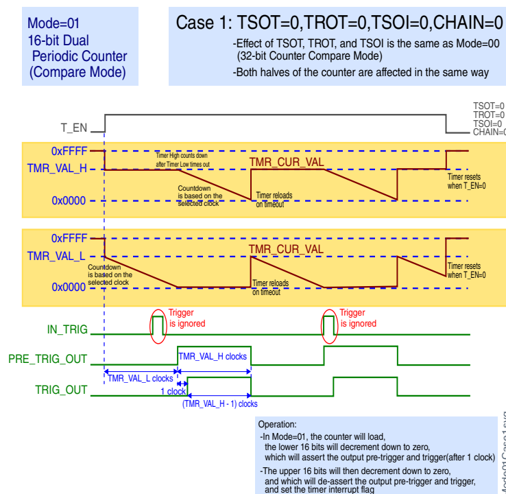
Figure 42-13. Case 1: TSOT = 0, TROT = 0, TSOI = 0, CHAIN = 0
