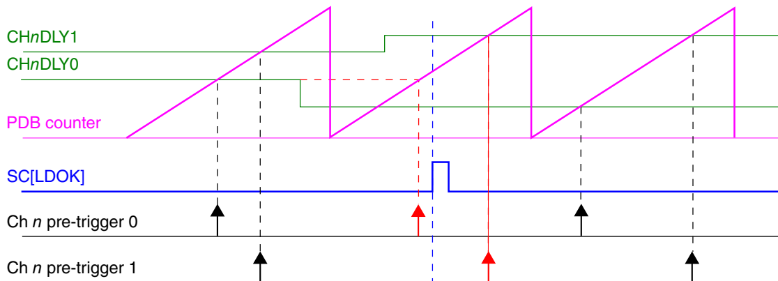
Figure 40-10. Registers update with SC[LDMOD] = 00
