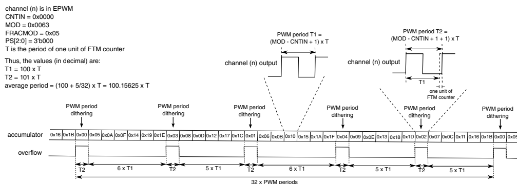
Figure 41-118. Example of Average Period when the PWM Period Dithering is used with the Up Counting
