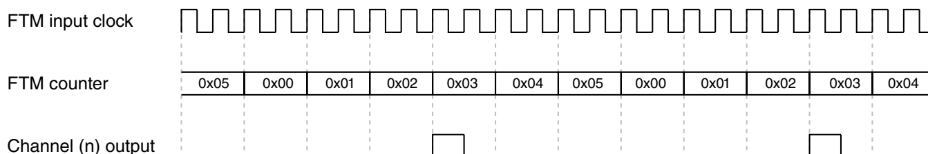
Figure 41-114. Example of channel (n) trigger at the channel (n) output in EPWM mode
