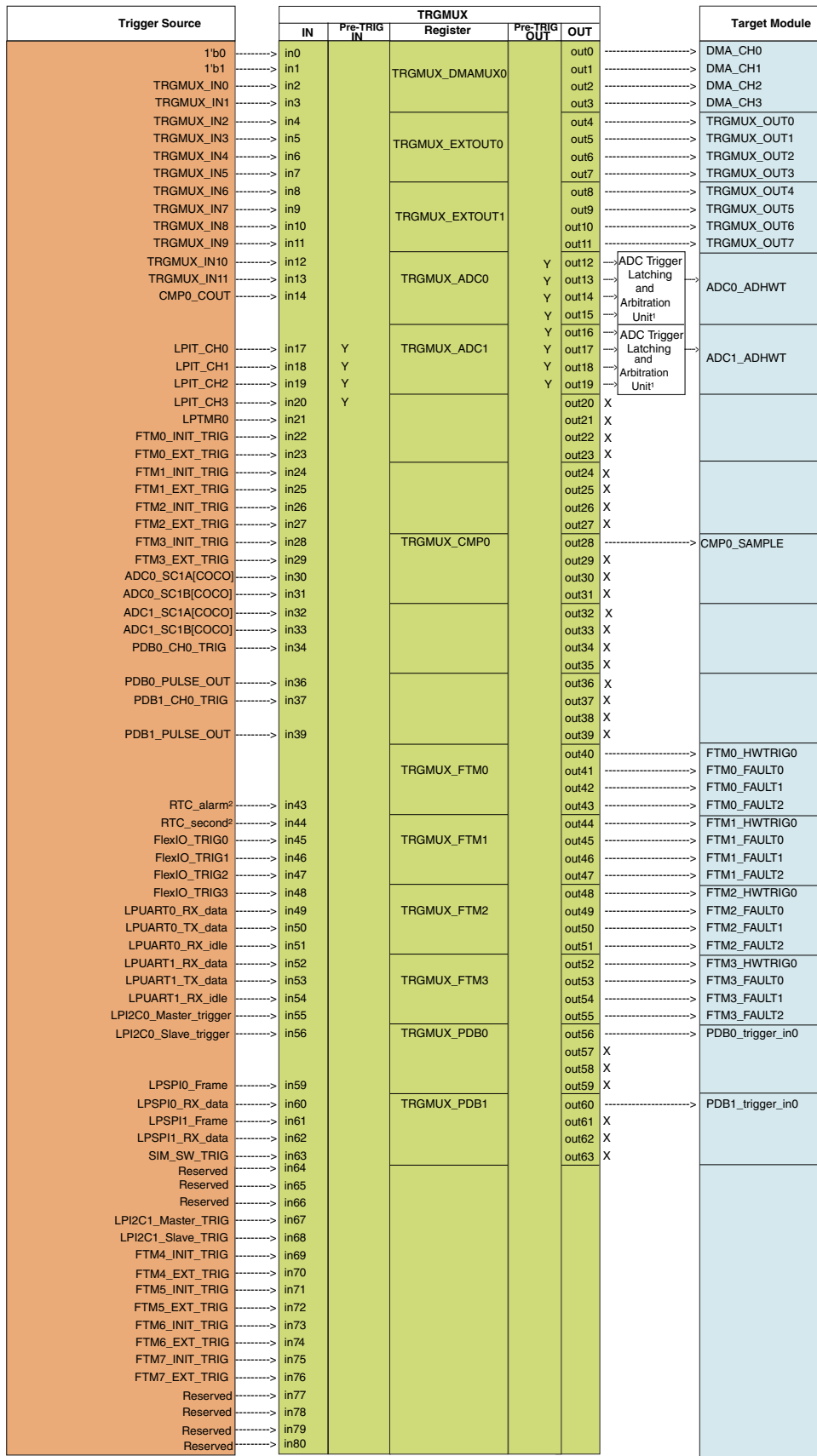
Figure 17-2. Trigger interconnectivity (part 1 of 2: outputs 0-63) MCXE24x Series Reference Manual, Rev. 2, 06/2025
