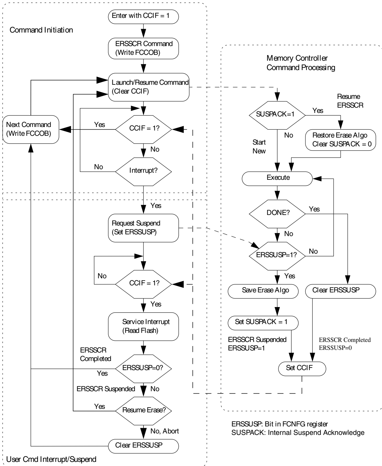
Figure 32-11. Suspend and resume of Erase Flash Sector operation
