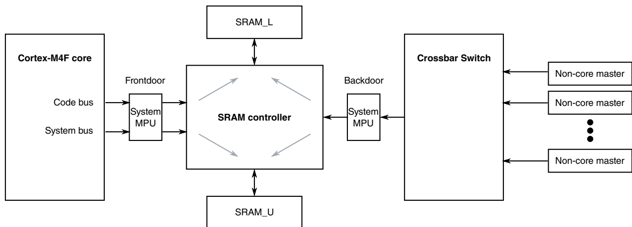
Figure 28-1. SRAM accessibility
