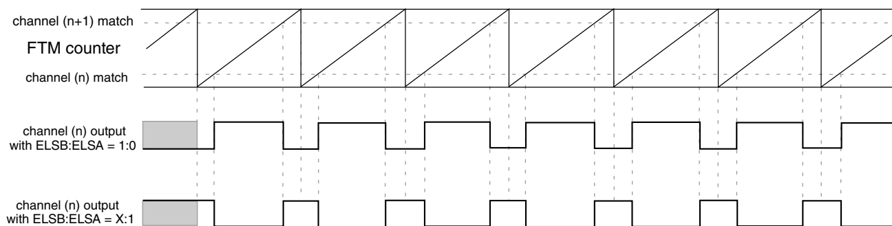
Figure 41-47. Modified Combine PWM Mode
