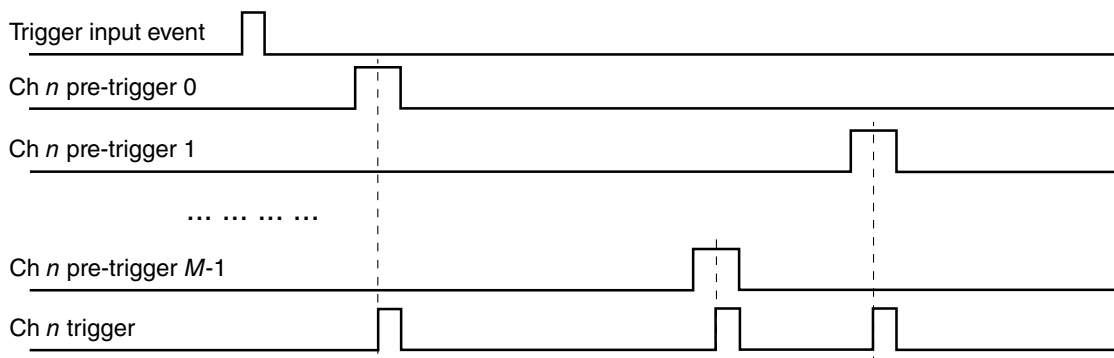
Figure 40-8. Pre-trigger and trigger outputs
