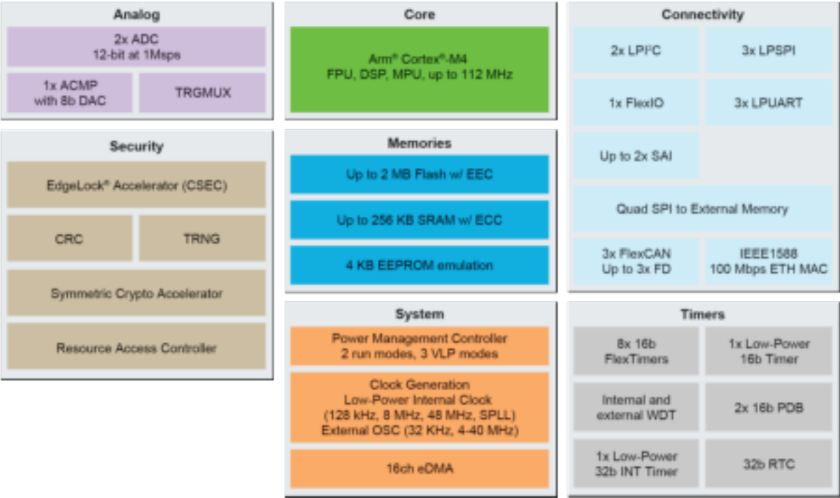
Figure 2-1. MCXE24x product series block diagram
