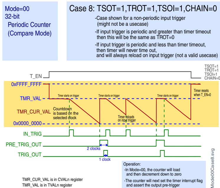
Figure 42-12. Case 8: TSOT = 1, TROT = 1, TSOI = 1, CHAIN = 0
