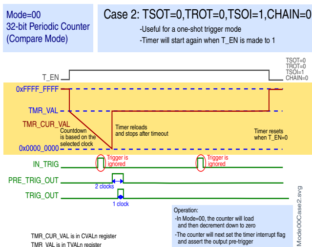
Figure 42-6. Case 2: TSOT = 0, TROT = 0, TSOI = 1, CHAIN = 0
