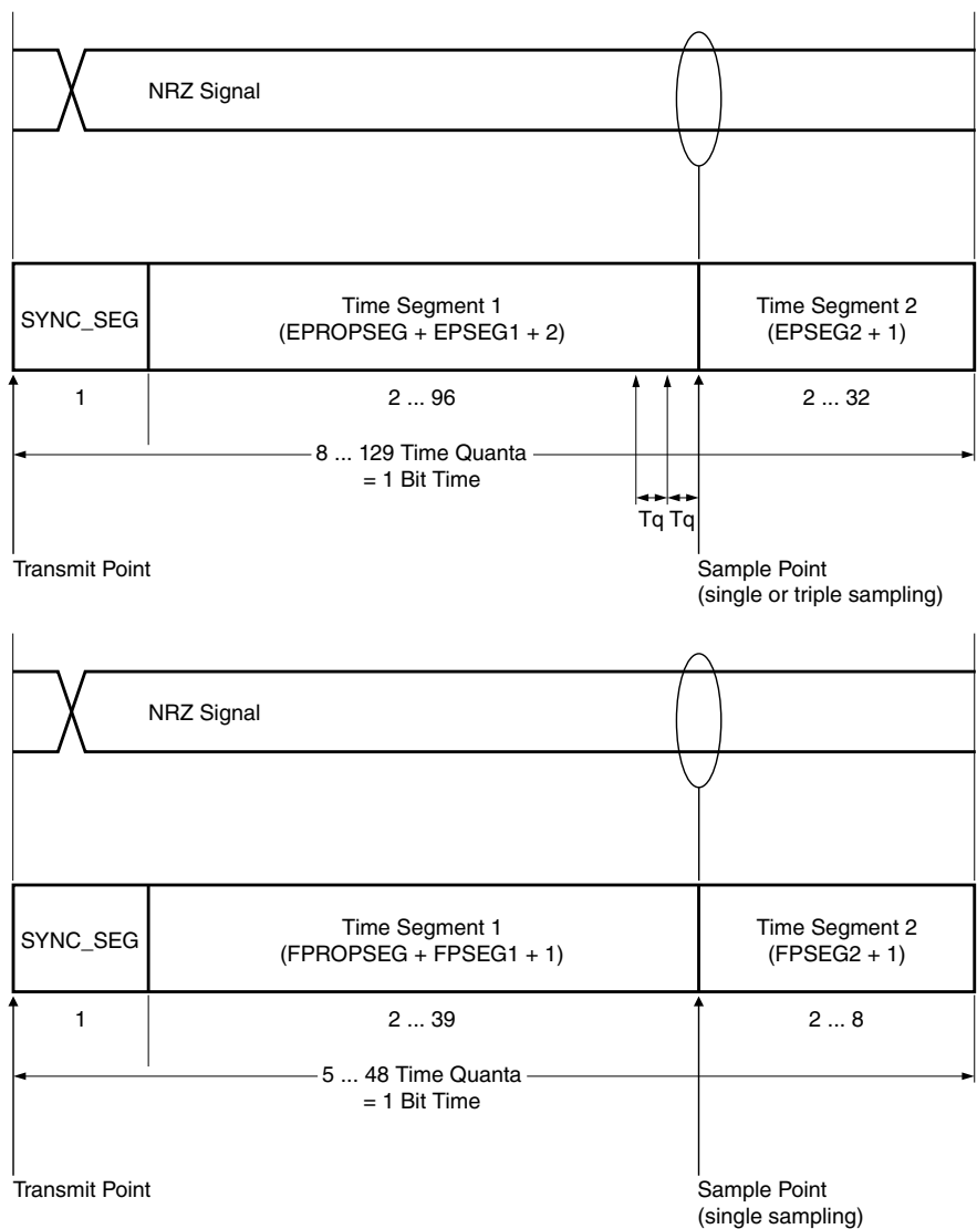
Figure 49-8. Segments within the bit time (example using CBT and FDCBT bit timing variables for CAN FD format)
