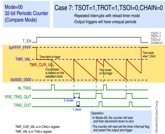
Figure 42-11. Case 7: TSOT = 1, TROT = 1, TSOI = 0, CHAIN = 0
