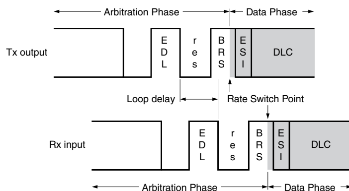
Figure 49-4. Transceiver loop delay measurement
