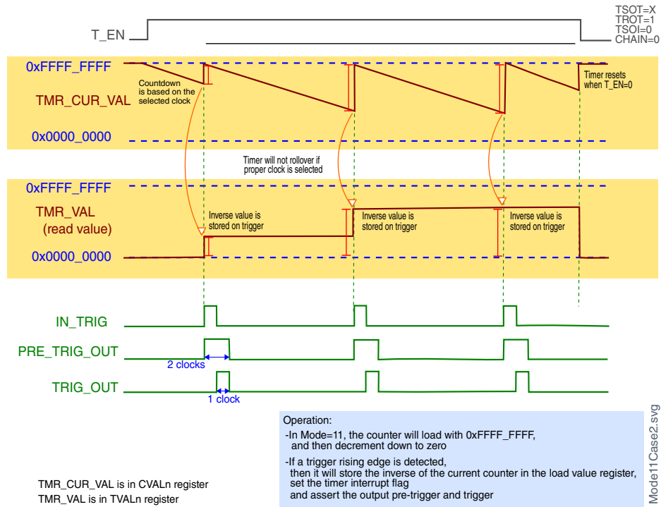
Figure 42-17. Case 2: TSOT = X, TROT = 1, TSOI = 0, CHAIN = 0
