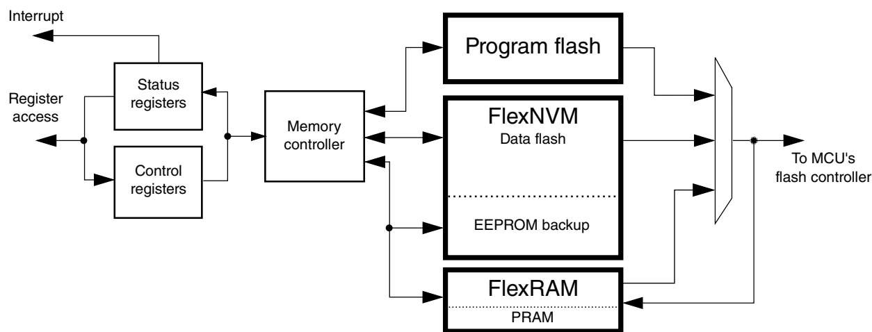
Figure 32-5. FTFC block diagram
