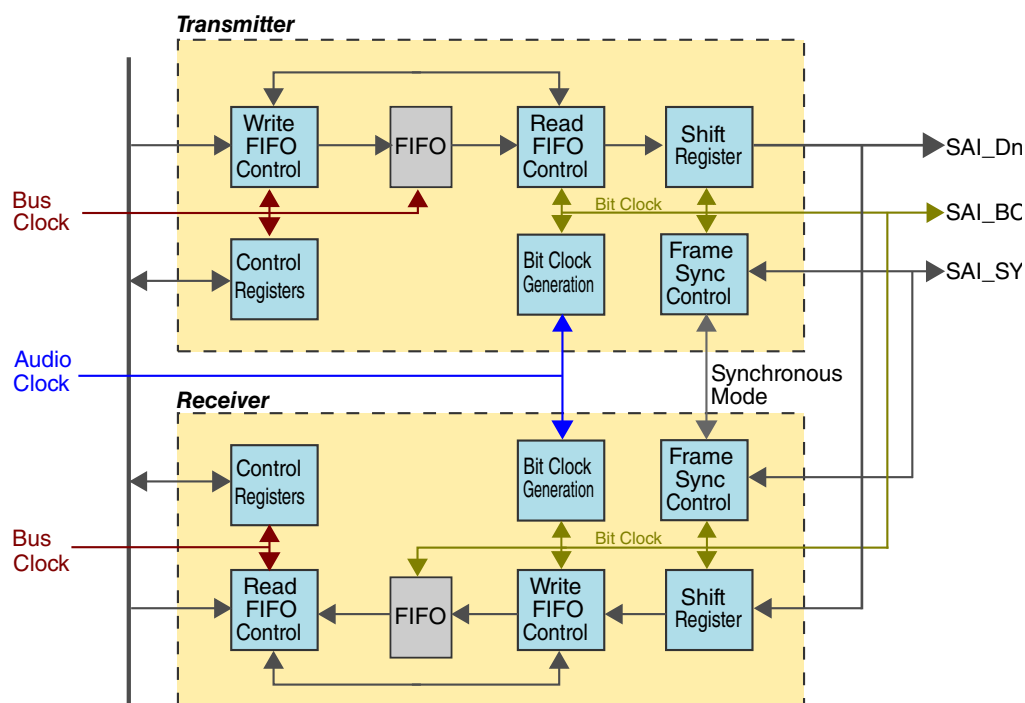
Figure 50-1. MCXE247 SAI Block Diagram
