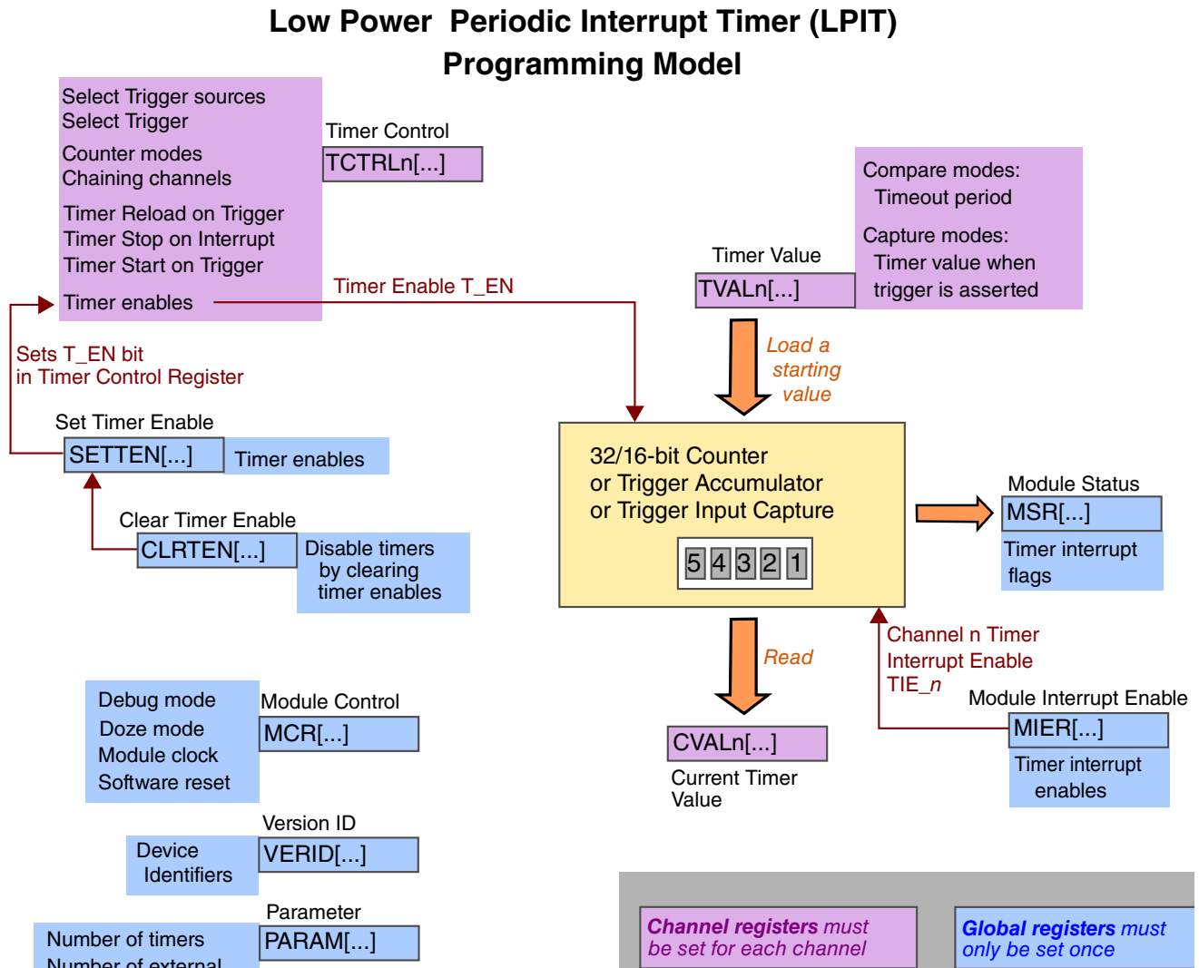
Figure 42-4. Programming Model
