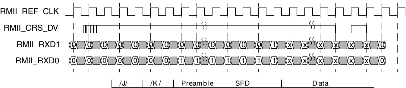
Figure 51-19. RMII receive operation
