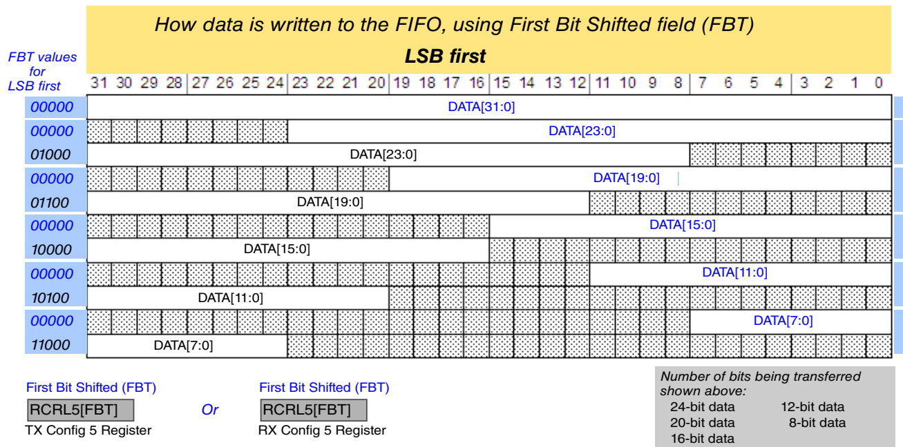
Figure 50-3. SAI first bit shifted, LSB first
