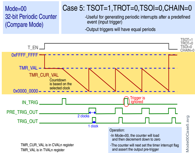
Figure 42-9. Case 5: TSOT = 1, TROT = 0, TSOI = 0, CHAIN = 0
