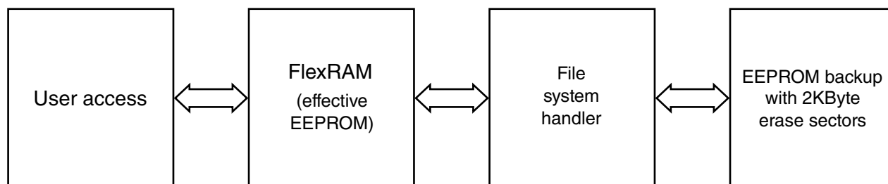
Figure 32-9. Top-level emulated EEPROM architecture
