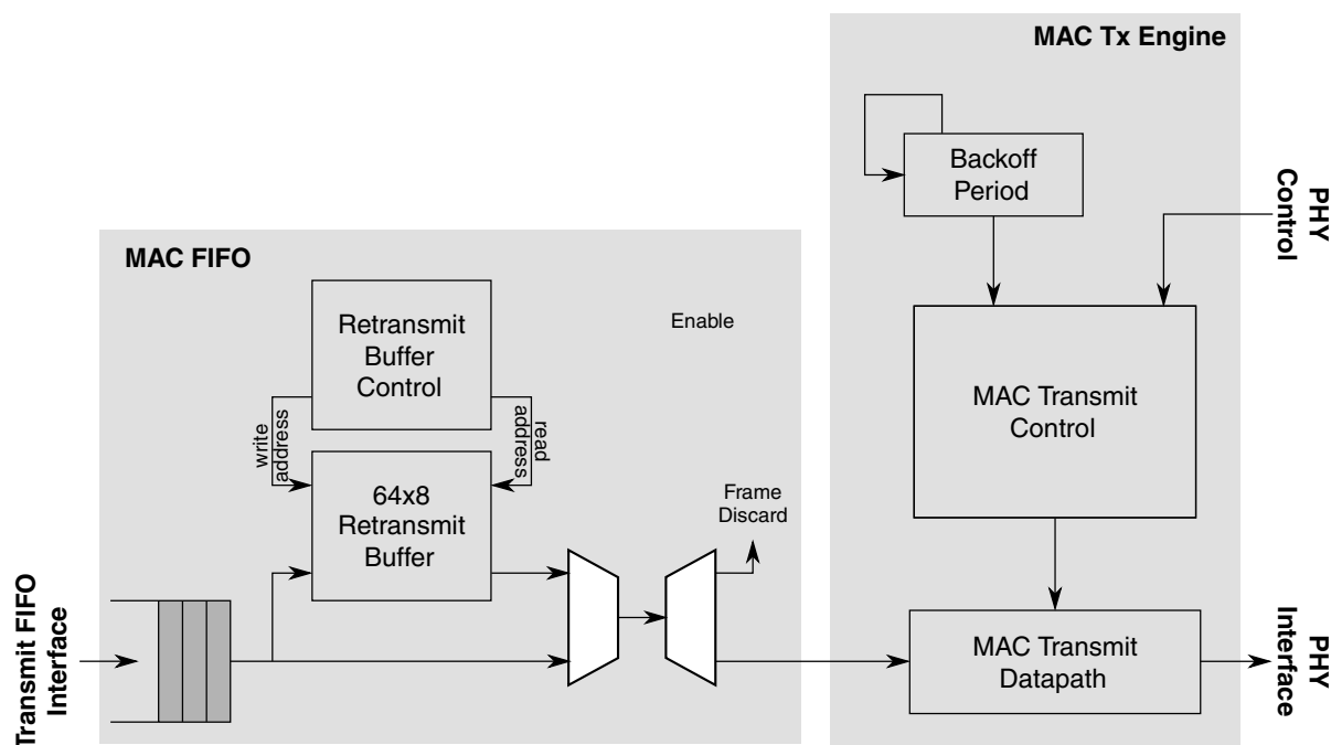
Figure 51-7. Packet re-transmit overview
