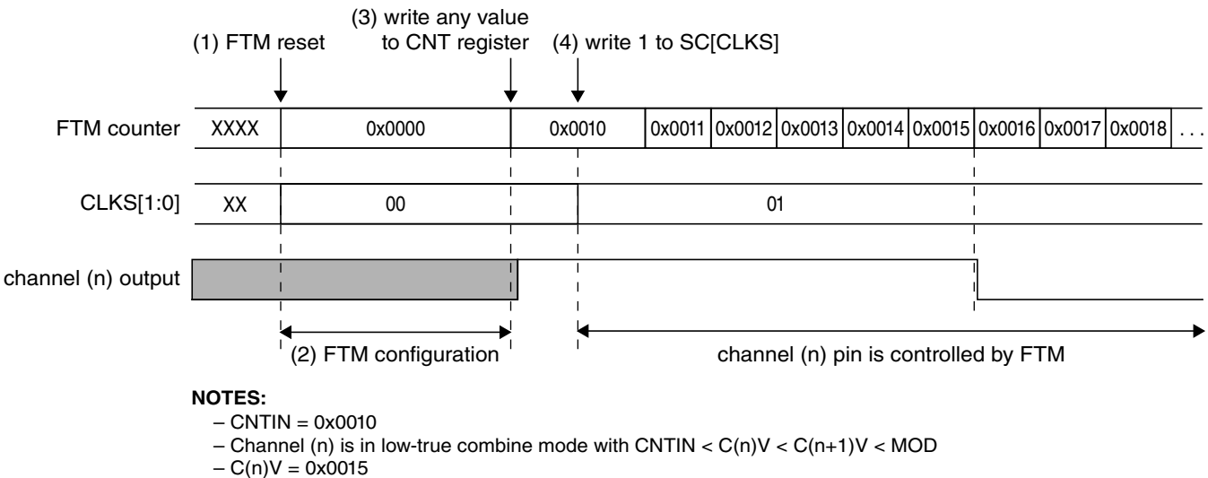
Figure 41-127. FTM behavior after reset when the channel (n) is in Combine mode
