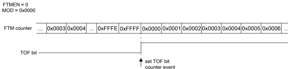
Figure 41-13. Example when the FTM counter is free running
