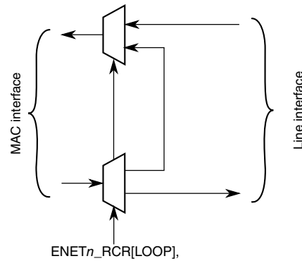
Figure 51-13. Loopback options
