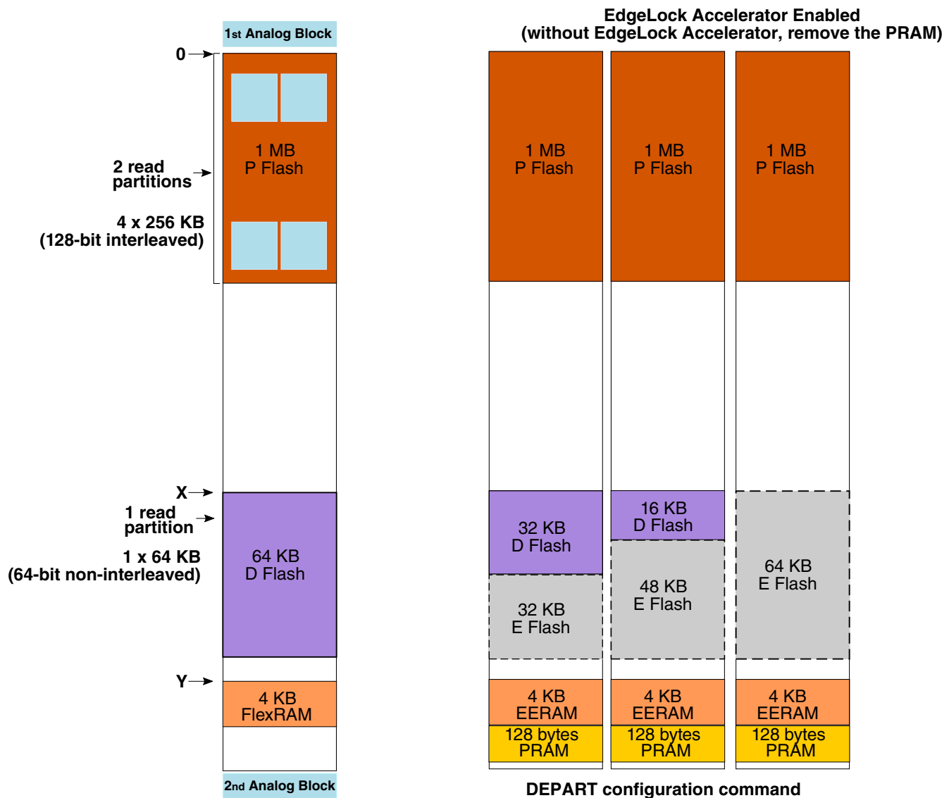
Figure 32-2. 1 MB flash memory map
