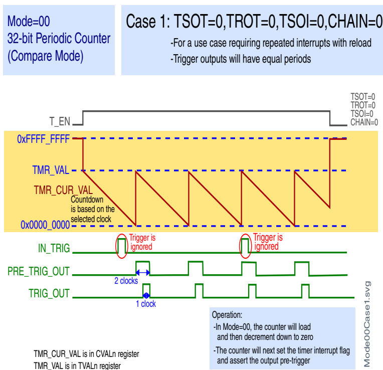
Figure 42-5. Case 1: TSOT = 0, TROT = 0, TSOI = 0, CHAIN = 0
