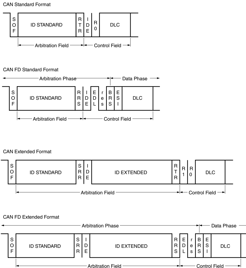
Figure 49-2. CAN message formats
