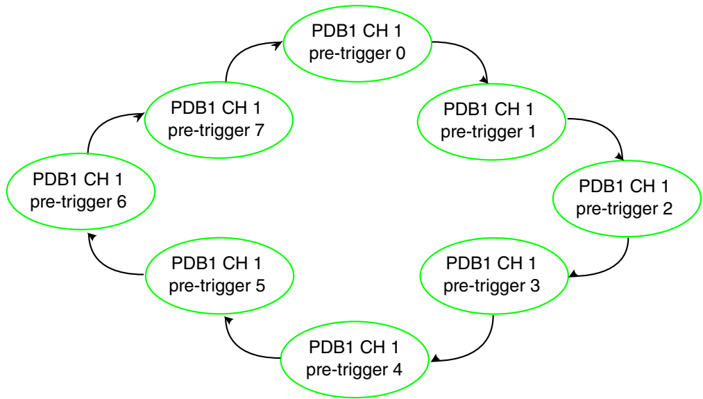
Figure 40-2. Example: PDB1 CH1 back-to-back chain
