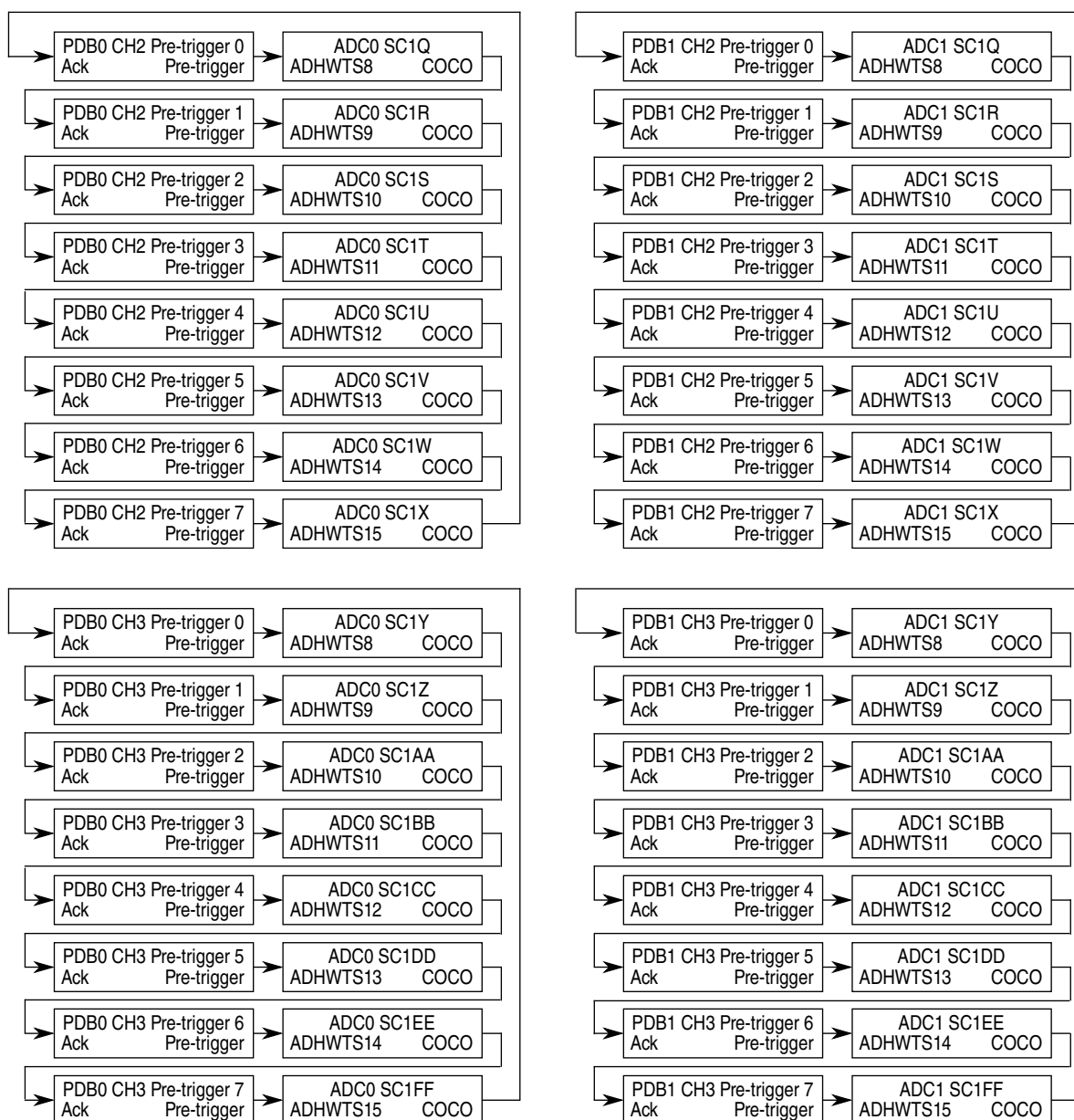
Figure 40-6. PDB-ADC back to back connection (Part 2 of 2)
