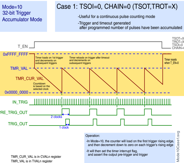
Figure 42-14. Case 1: TSOT = X, TROT = X, TSOI = 0, CHAIN = 0
