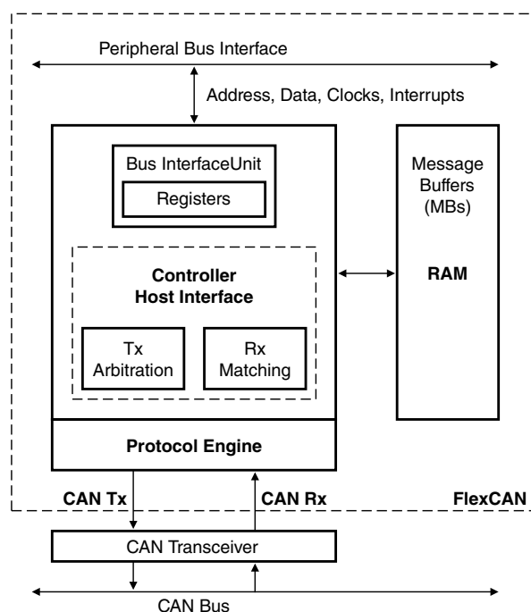
Figure 49-1. FlexCAN block diagram
