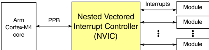
Figure 7-2. NVIC configuration
