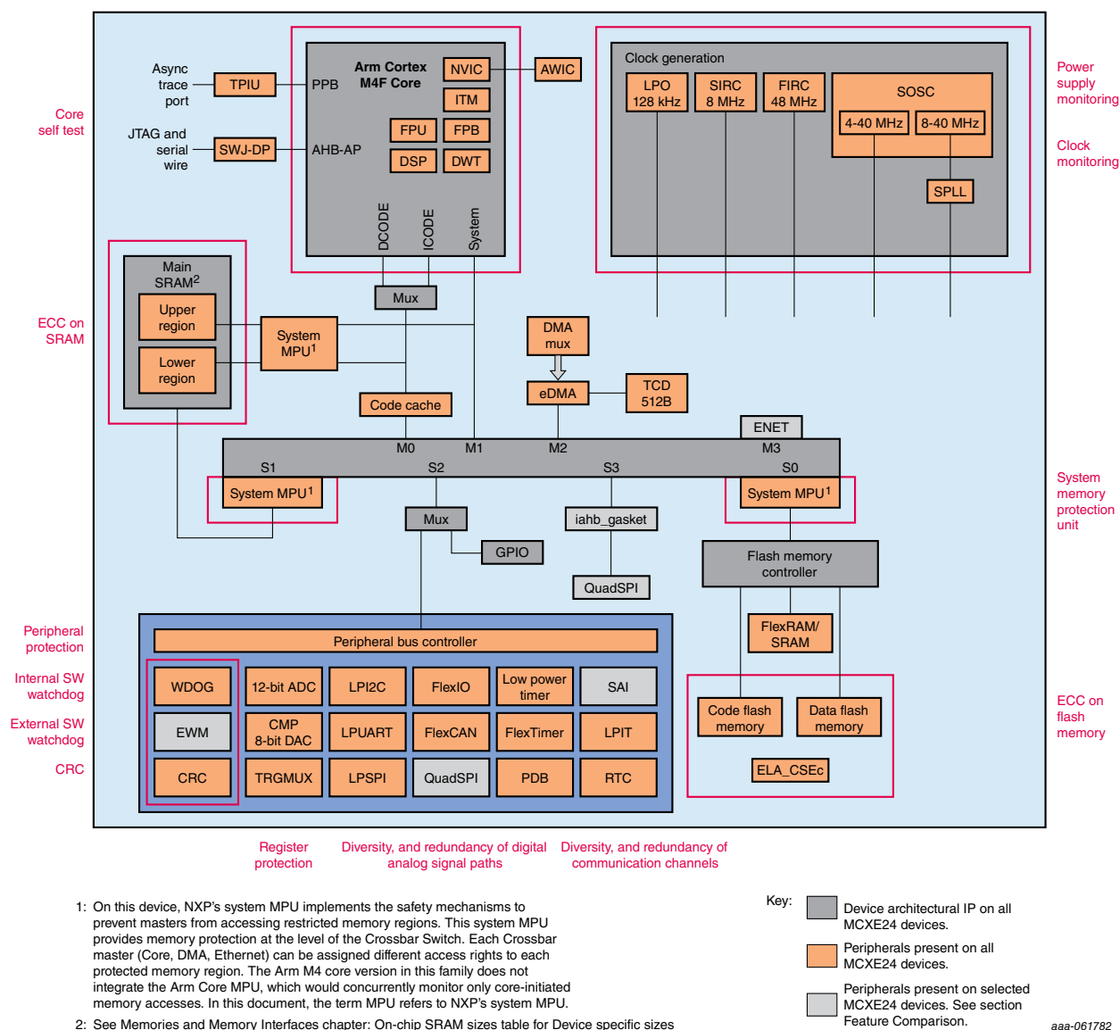
Figure 6-2. MCXE24x safety block diagram
