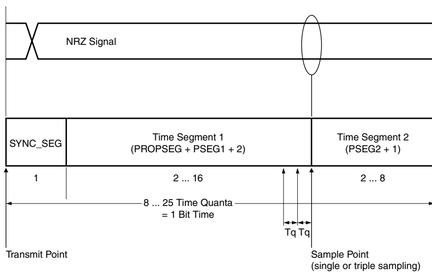
Figure 49-7. Segments within the bit time (example using CTRL1 bit timing variables for Classical CAN format)
