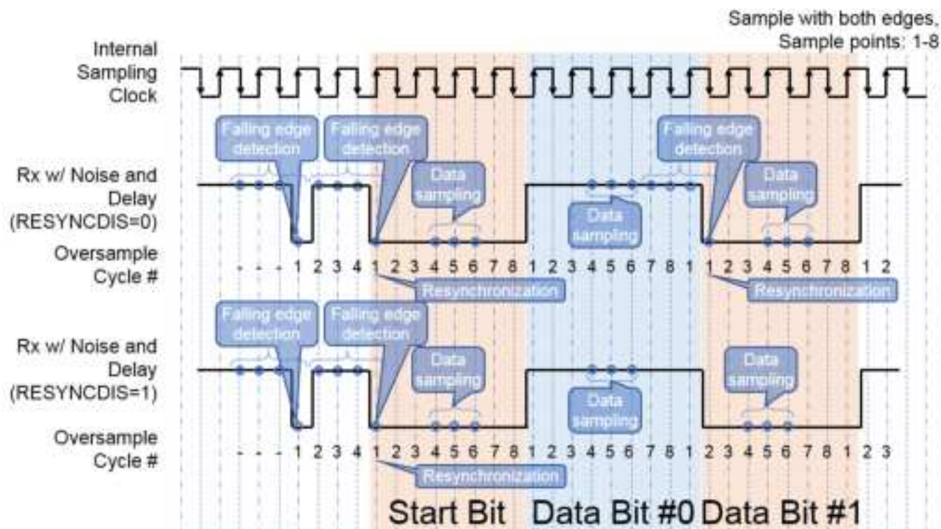
Figure 47-5. LPUART resynchronization
