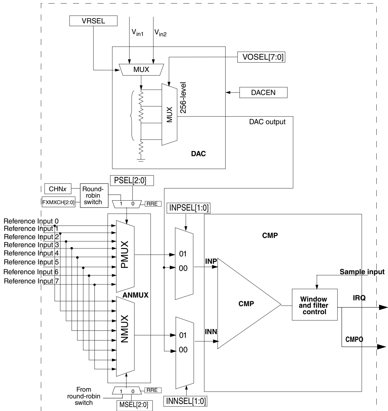
Figure 39-1. CMP high level diagram
