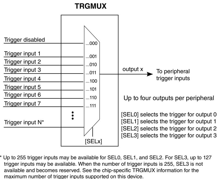
Figure 17-4. TRGMUX block diagram
