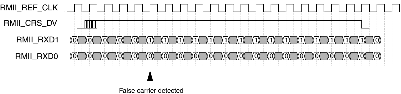
Figure 51-20. RMII receive operation with false carrier
