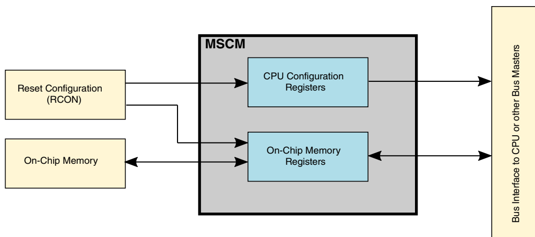
Figure 30-1. MSCM Block Diagram
