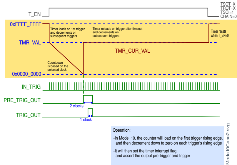
Figure 42-15. Case 2: TSOT = X, TROT = X, TSOI = 1, CHAIN = 0
