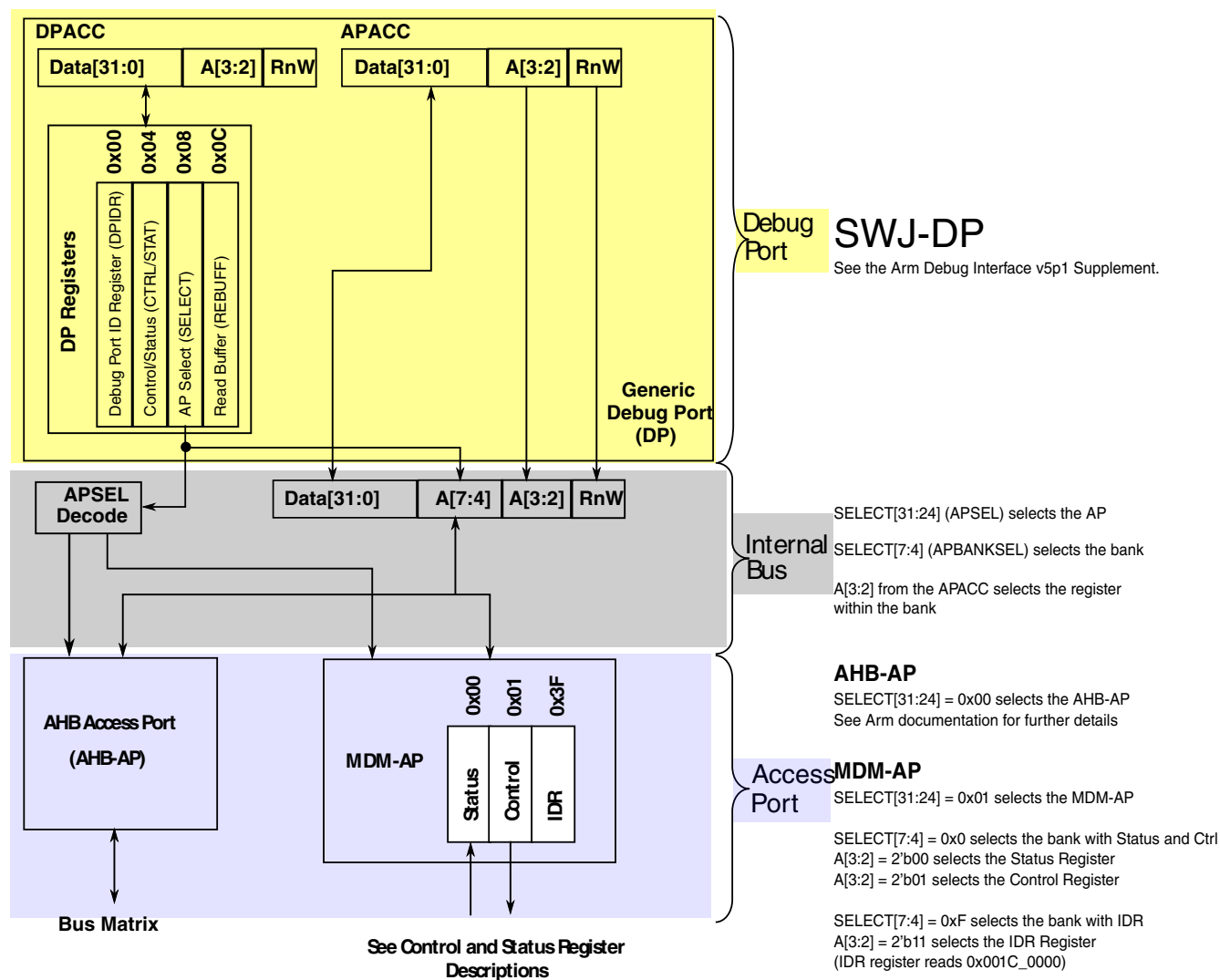
Figure 52-3. MDM AP addressing
