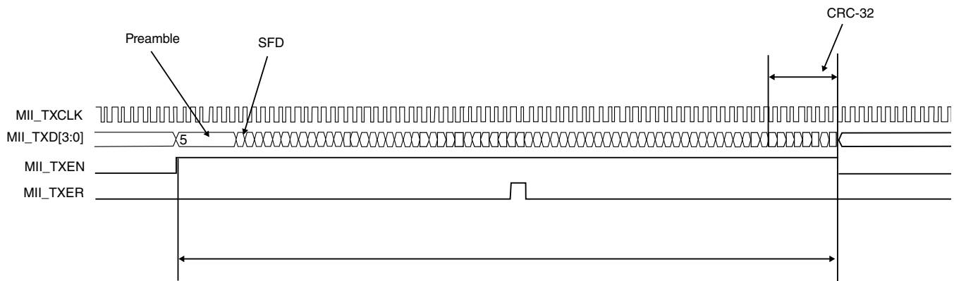
Figure 51-23. MII transmit operation — errored frame
