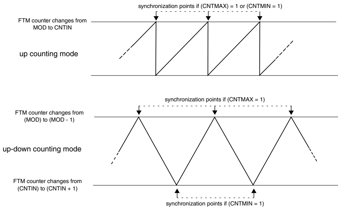
Figure 41-54. Synchronization Points
