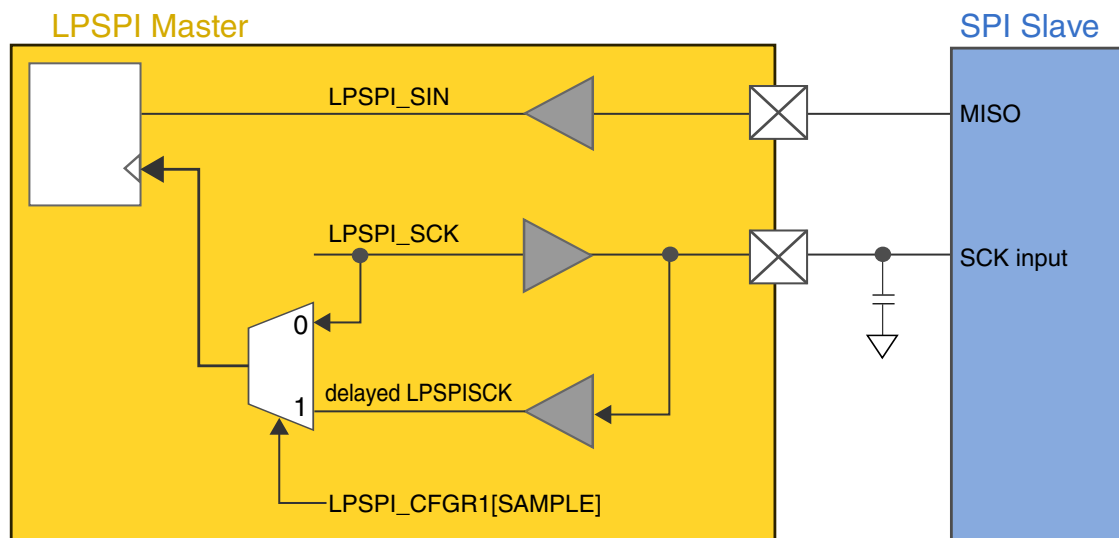
Figure 45-2. Clock Loopback
