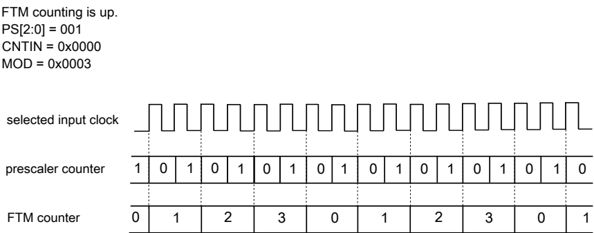
Figure 41-7. Example of the prescaler counter
