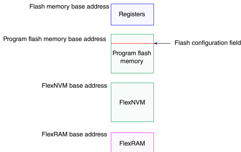
Figure 32-4. Flash memory map
