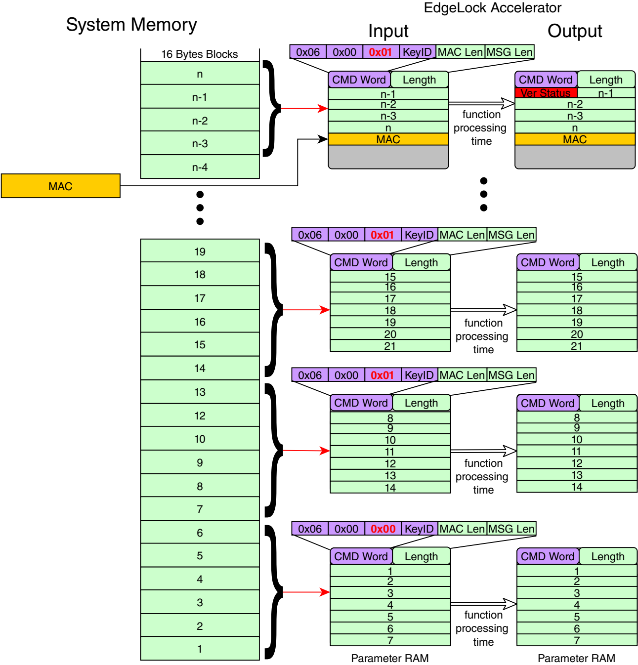
Figure 5-5. Message authentication
